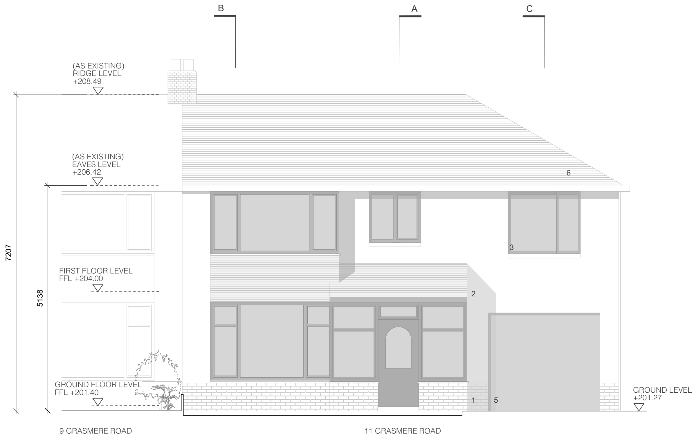
1 PROPOSED WEST ELEVATION 1:50 (A3)
