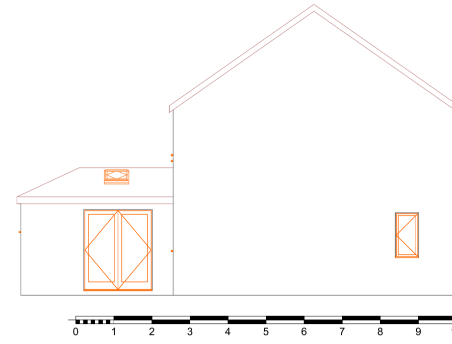
6 West Elevation Proposed 1:100
