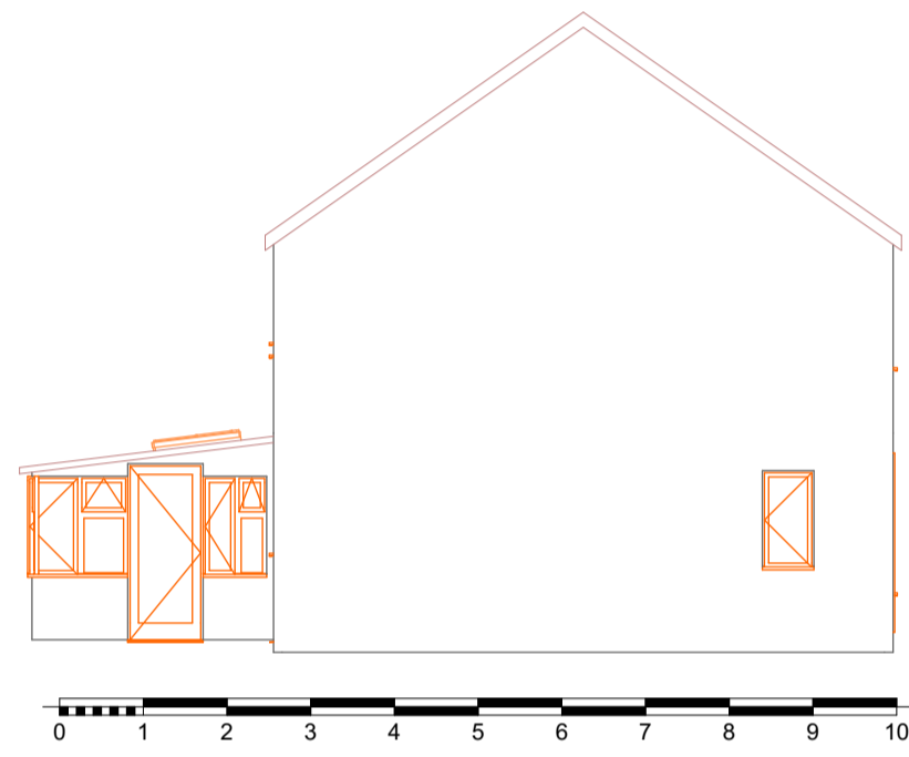
2 West Elevation Existing 1:100
