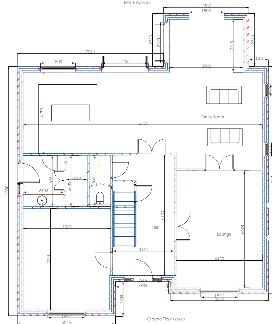
Ground Floor Layout
