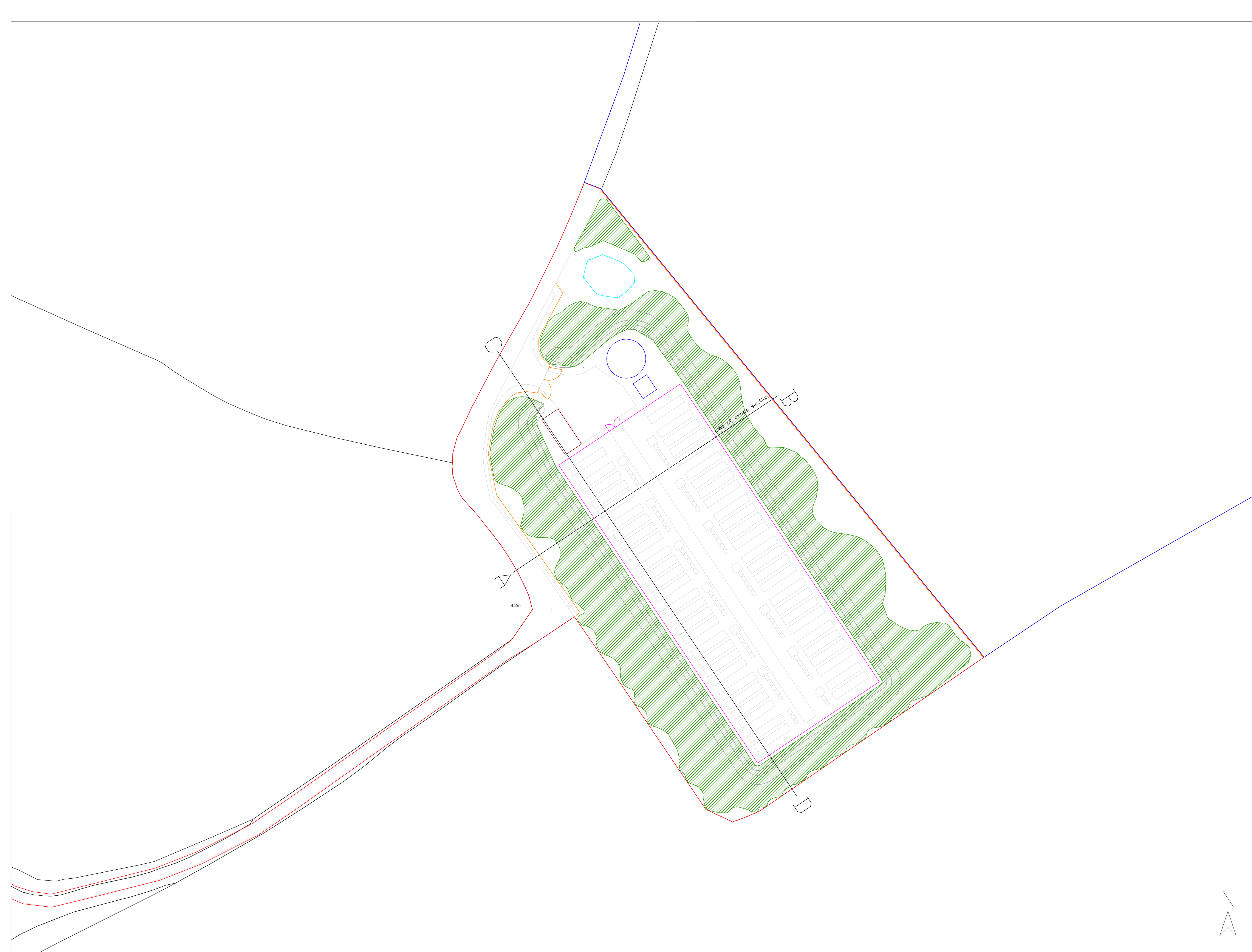
Figure 2. Proposed battery storage facility site layout
