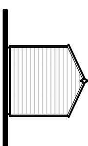
PROPOSED (EAST) ELEVATION (1:100)
