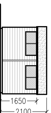
PROPOSED (NORTH) ELEVATION (1:100)
