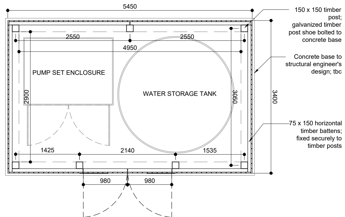
PLAN
