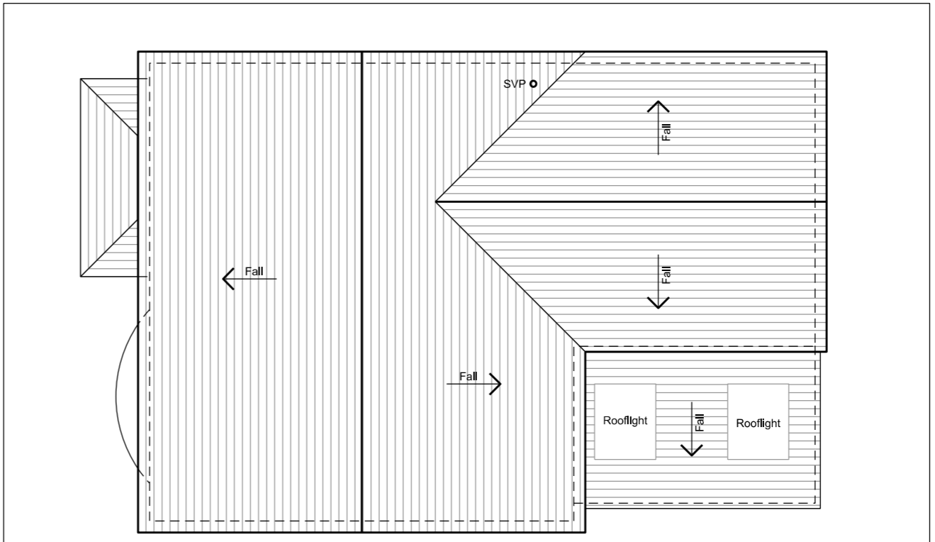
03 - Proposed Roof Plan 1:100@A3
