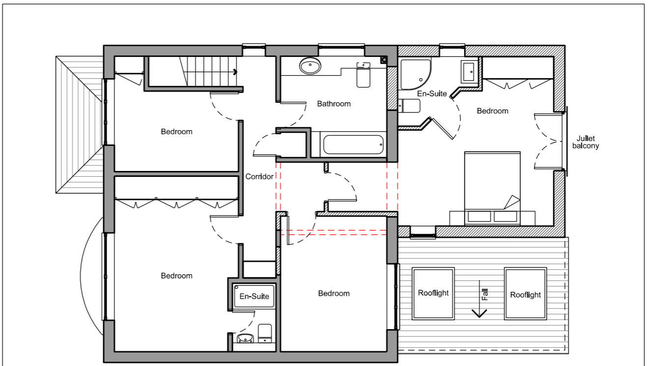
02 - Proposed First Floor Plan 1:100@A3
