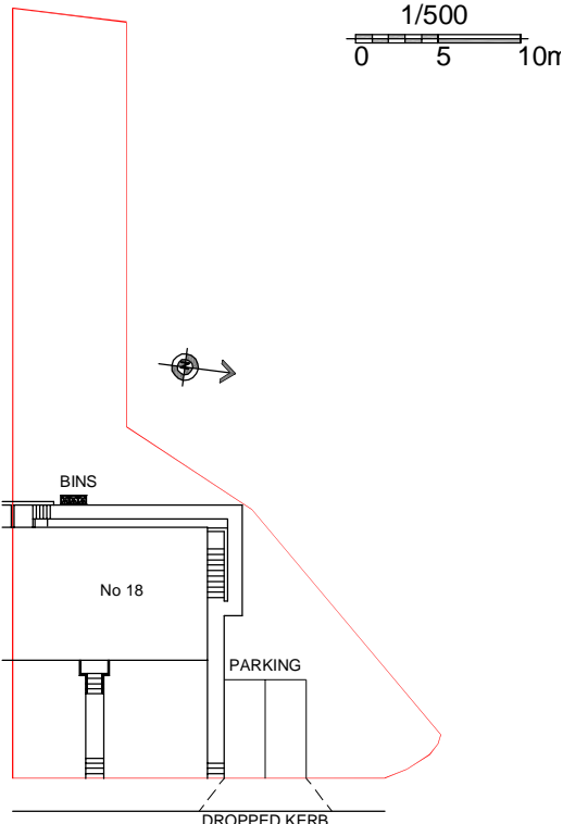
BLOCK PLAN AS PROPOSED
