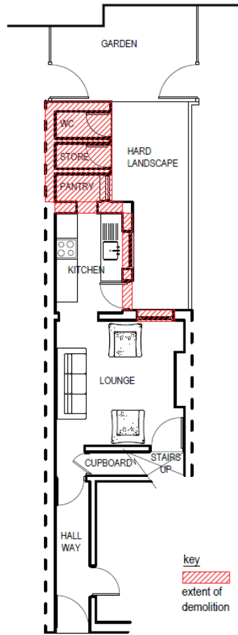
PROPOSED DEMOLITION PLAN 1:100@A3
