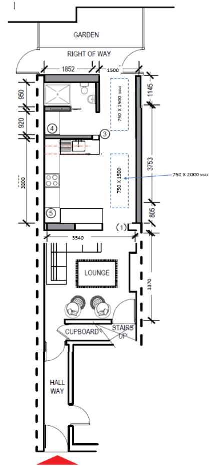
PROPOSED PLAN 1:100@A1
