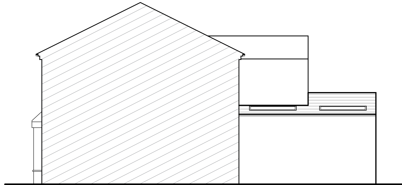
PROPOSED RIGHT ELEVATION (SECTION) 1:100@A3
