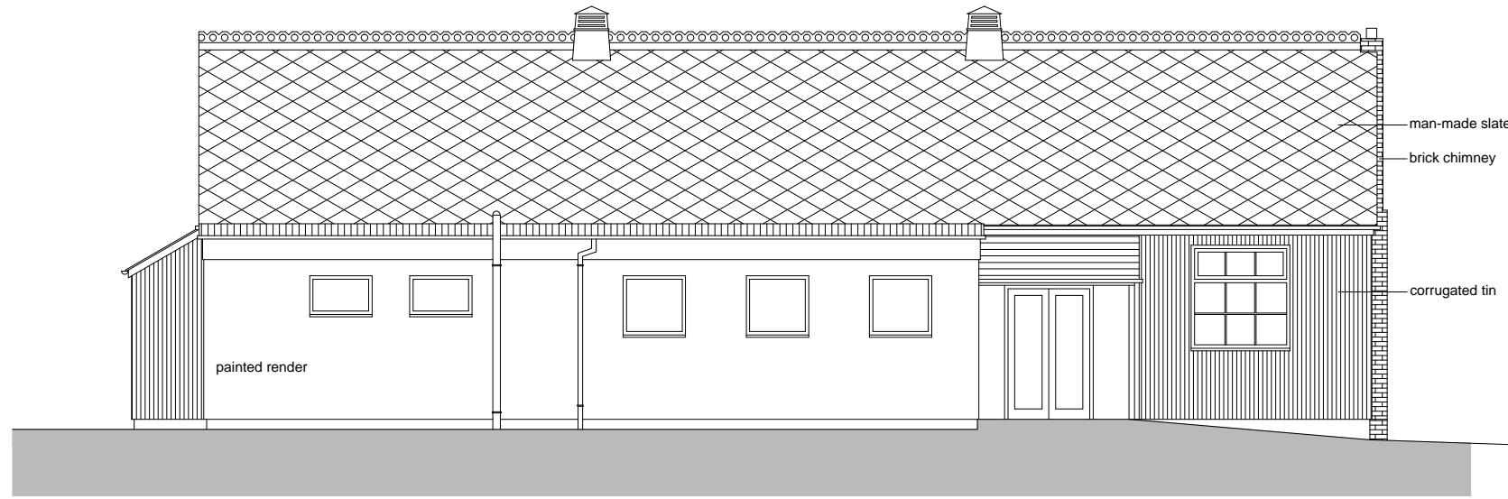
west elevation
