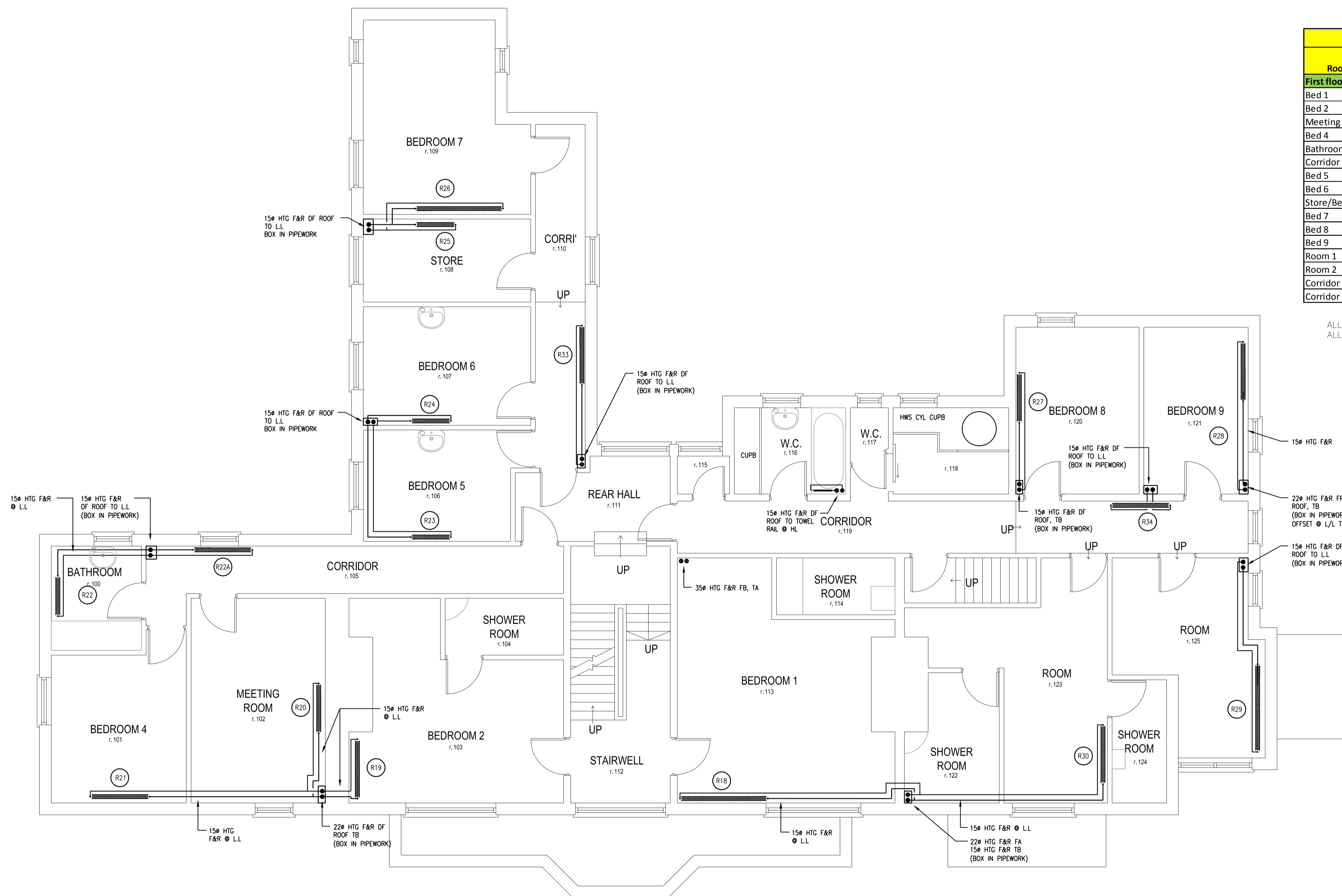
FIRST FLOOR @ 1:50
