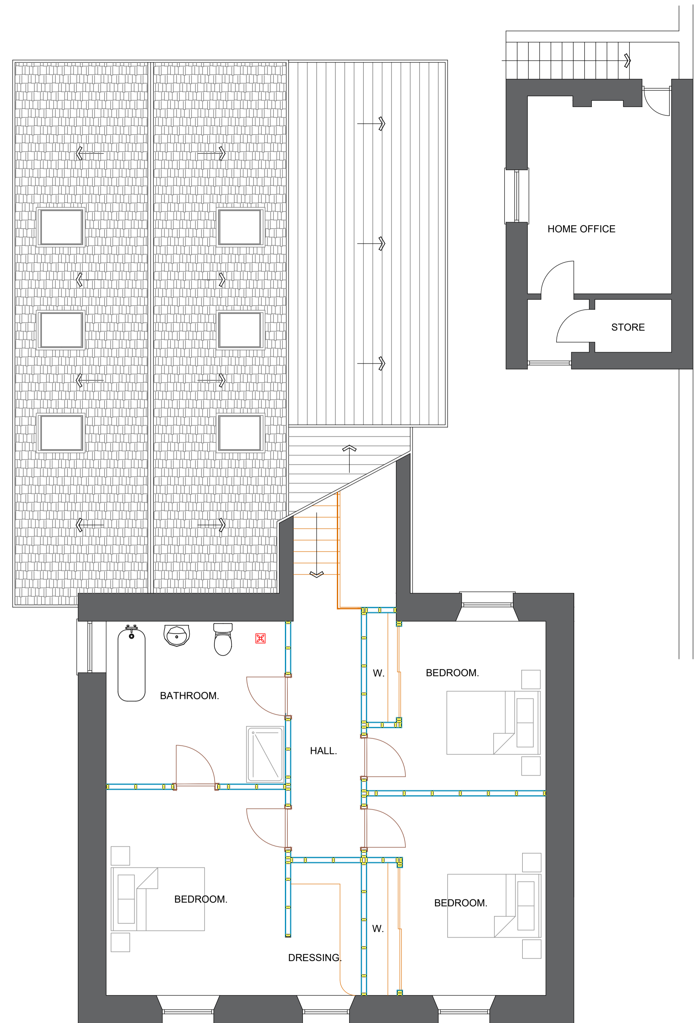
PROPOSED FIRST FLOOR LAYOUT
