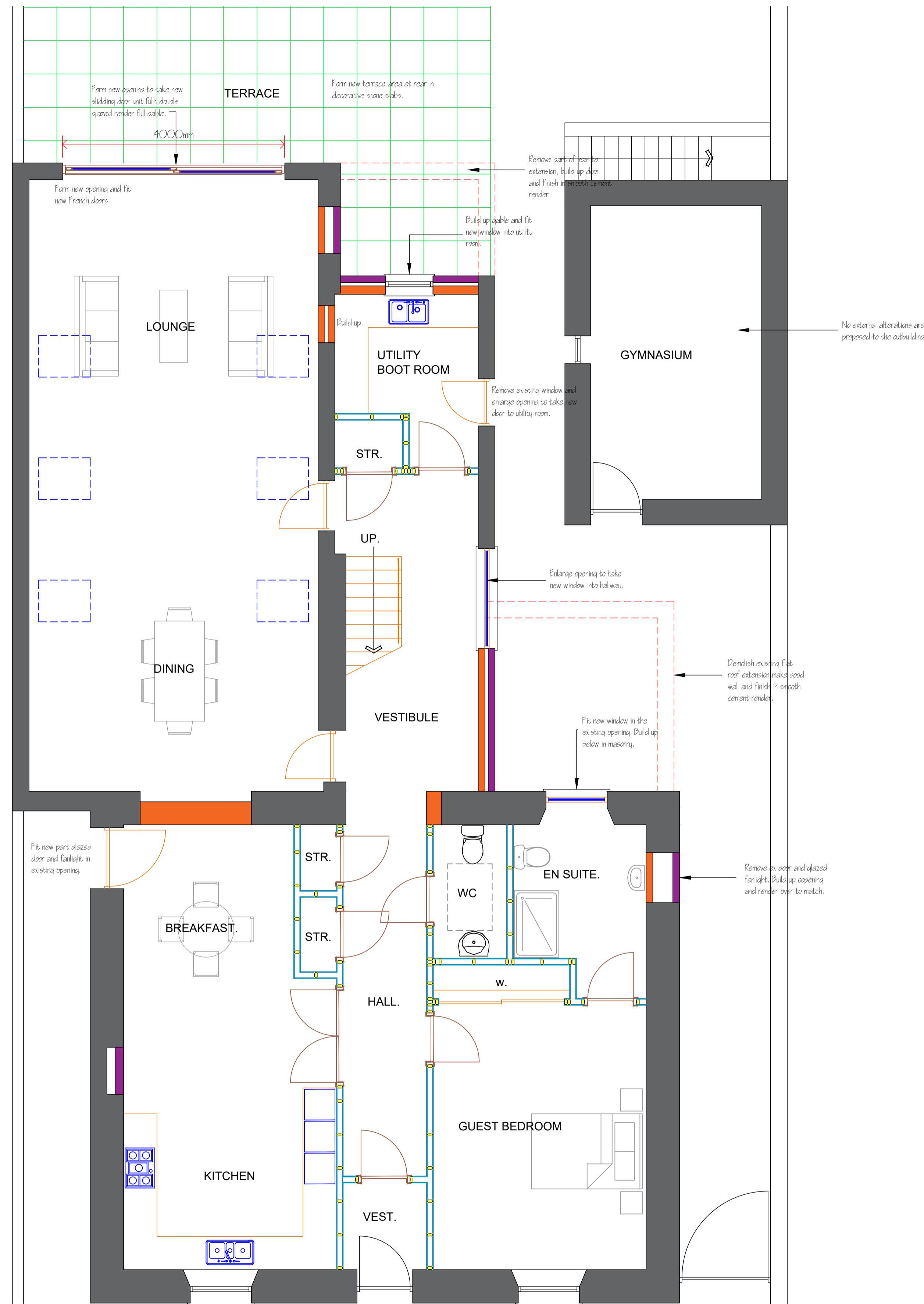
PROPOSED GROUND FLOOR LAYOUT
