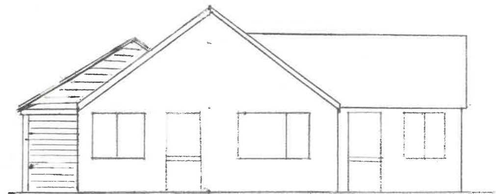
Rear Elevation North
