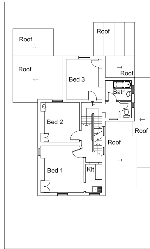
EXISTING FIRST FLOOR PLAN 1:200
