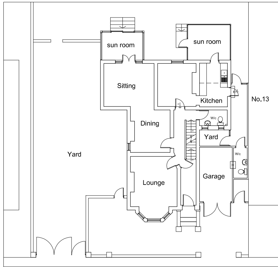
EXISTING GROUND FLOOR PLAN 1:200
