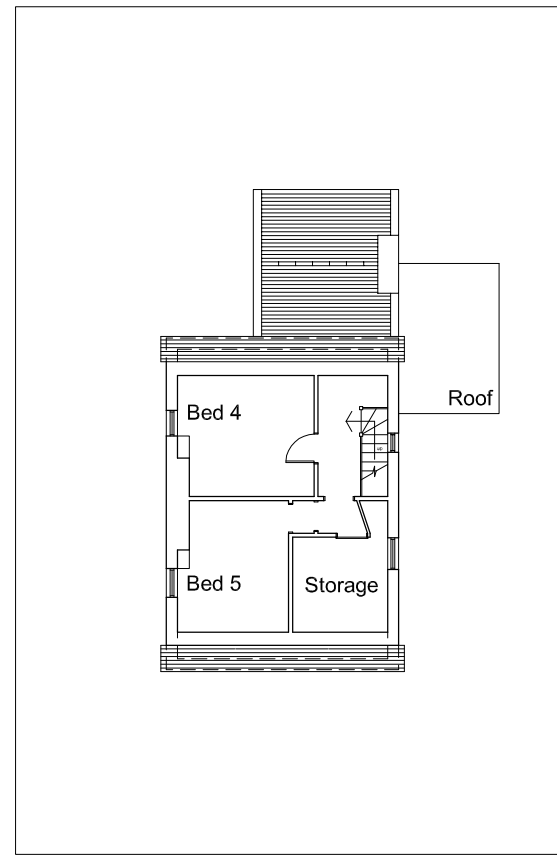
EXISTING SECOND FLOOR PLAN 1:200
