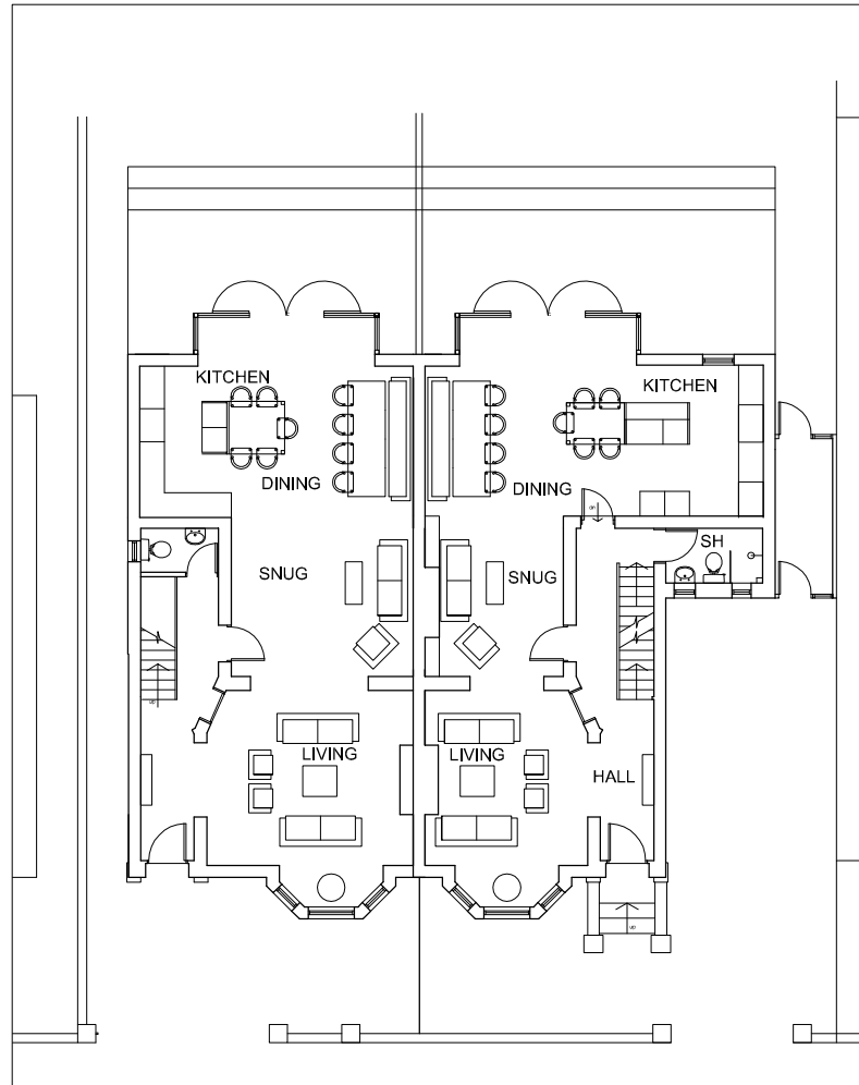
PROPOSED GROUND FLOOR PLAN 1:200
