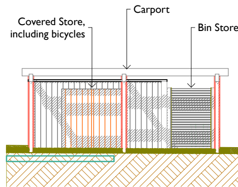
South-West Elevation
