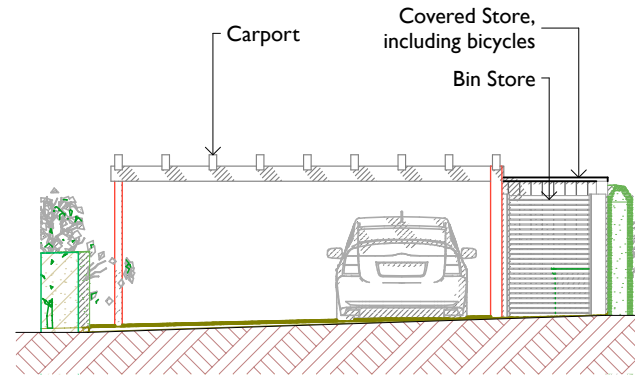
South-East Elevation
