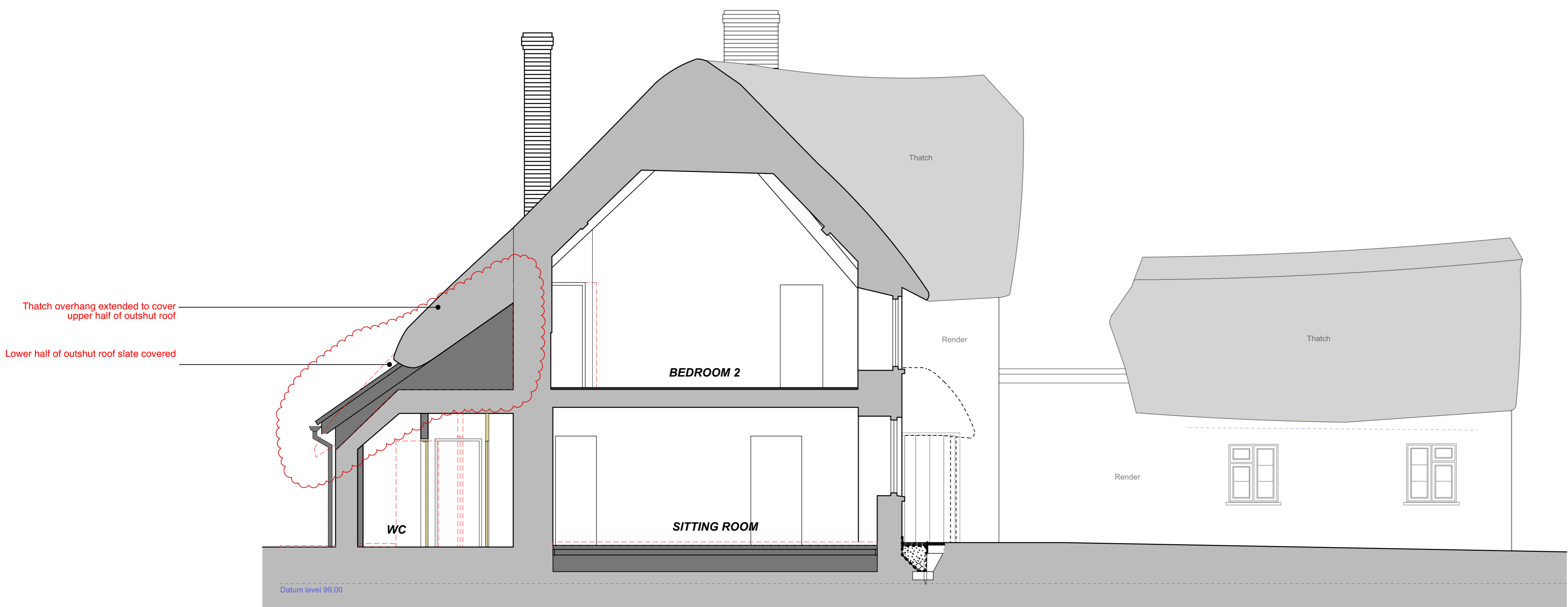
Proposed Section AA 1:50@A1, 1:100@A3
