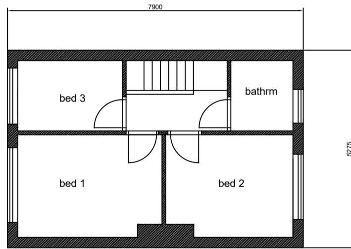
existing floor plan 1:100
