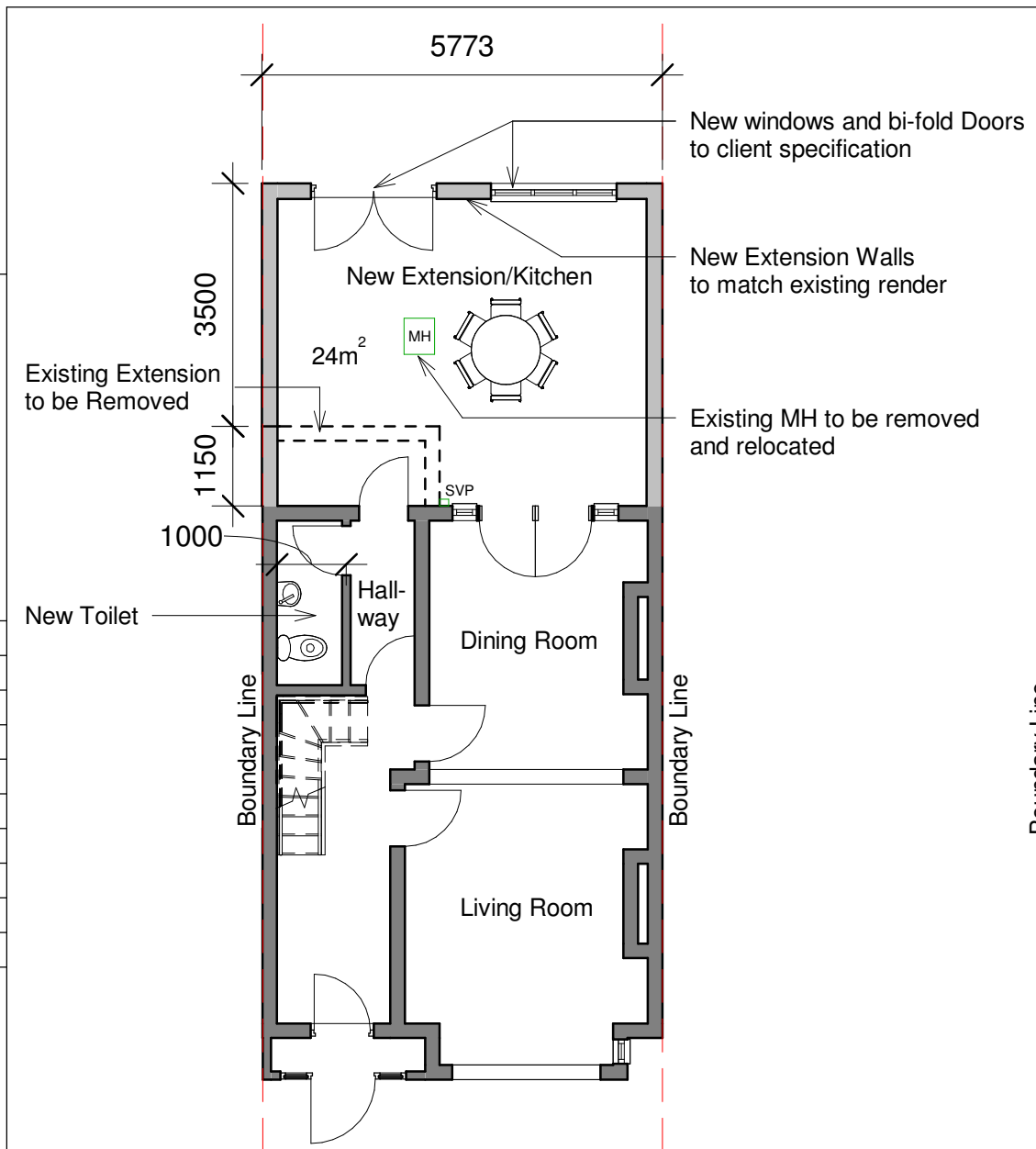
1 Proposed Ground Floor 1 : 100
