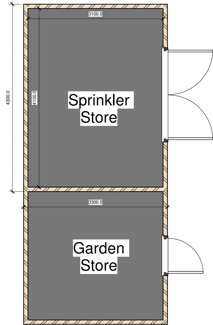
Plan View 1 : 50
