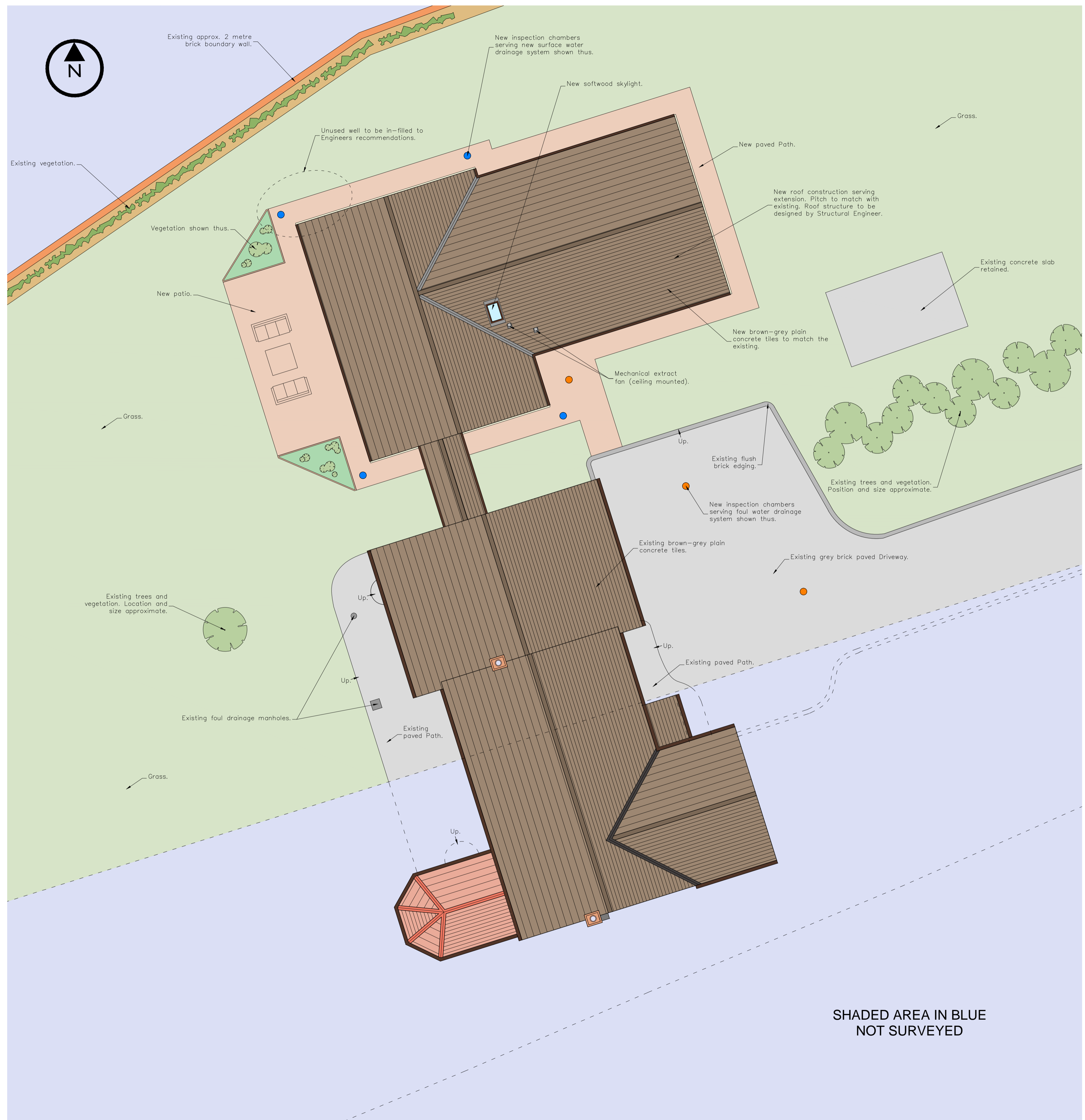
Proposed Roof Plan Scale 1:100
