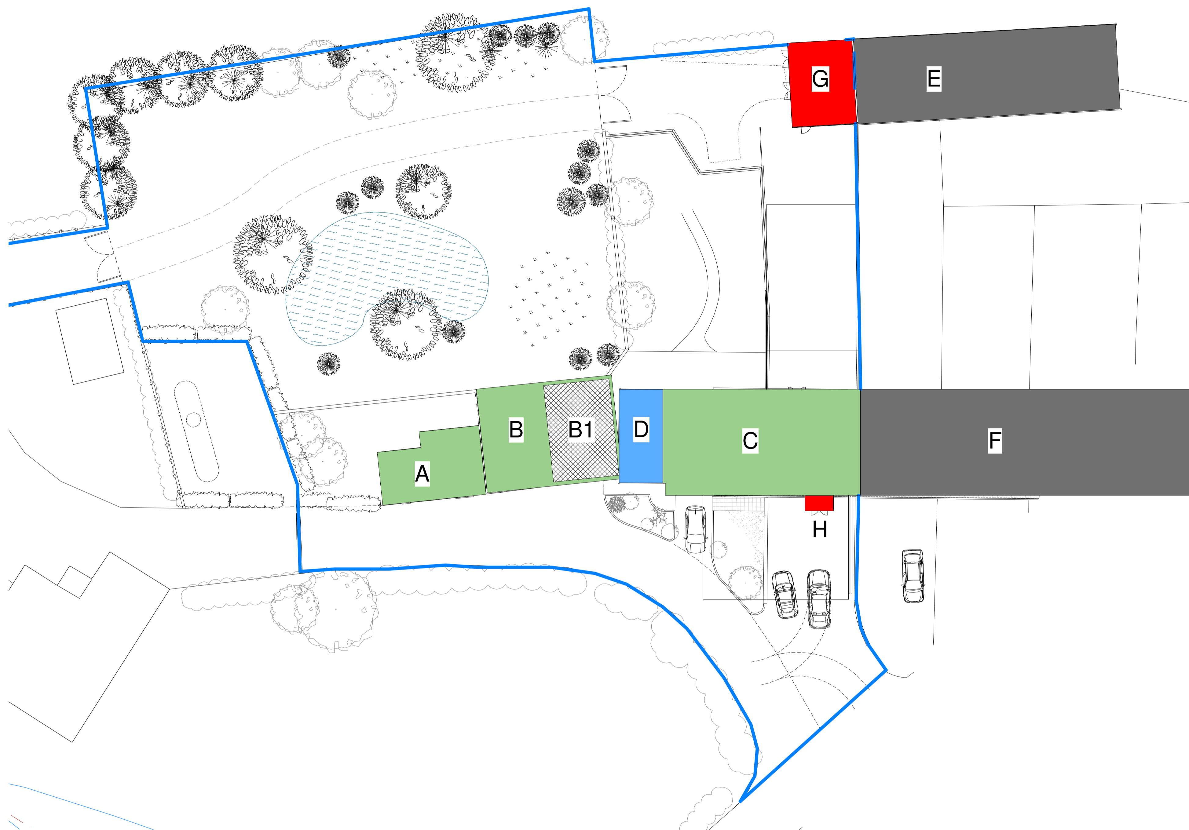
1 Site Plan - Original & Proposed Extension volumes 1 : 200
