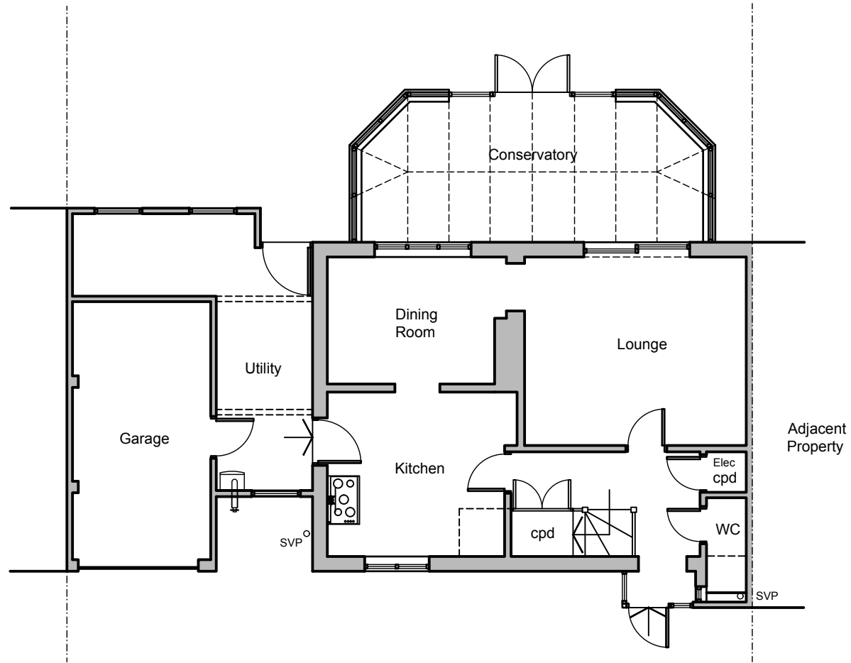
1. Ground Floor Plan
