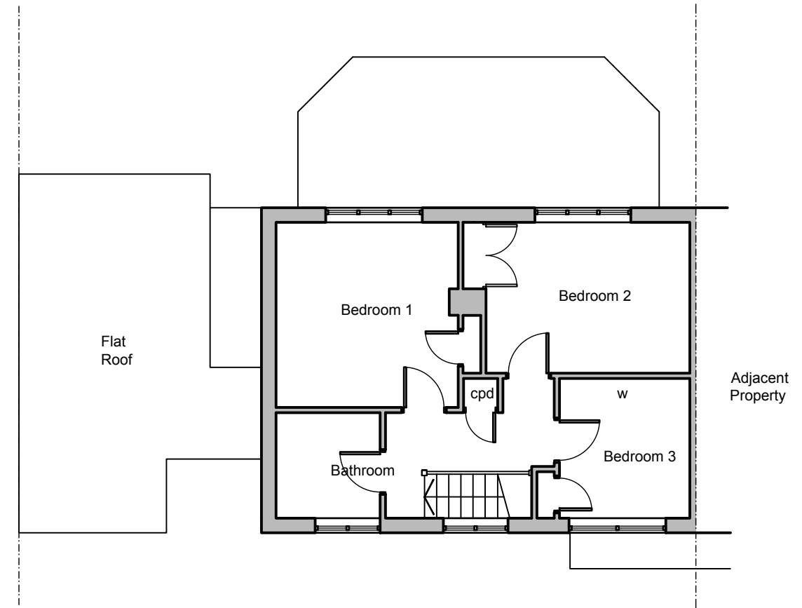
2. First Floor Plan
