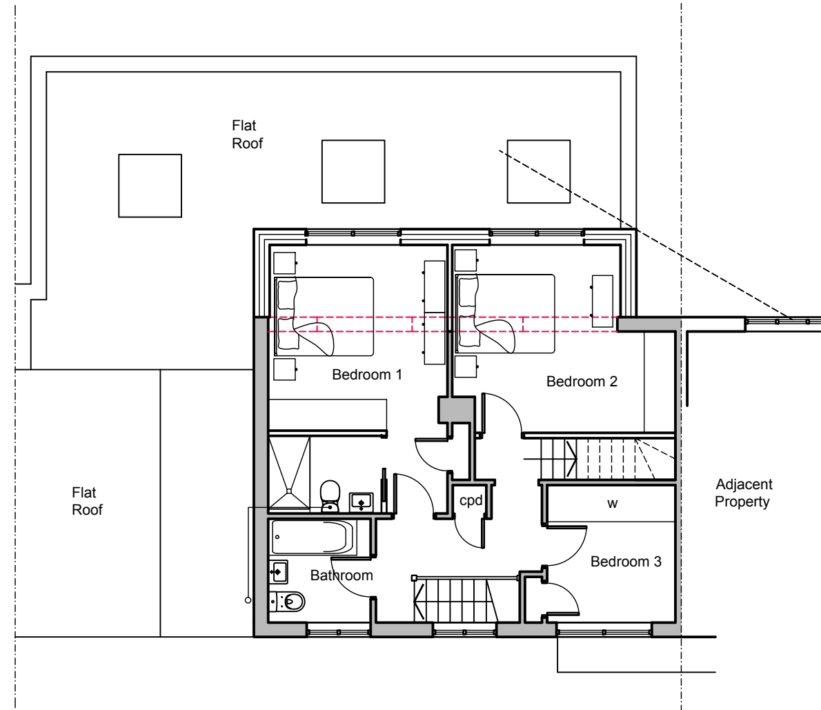
2. First Floor Plan
