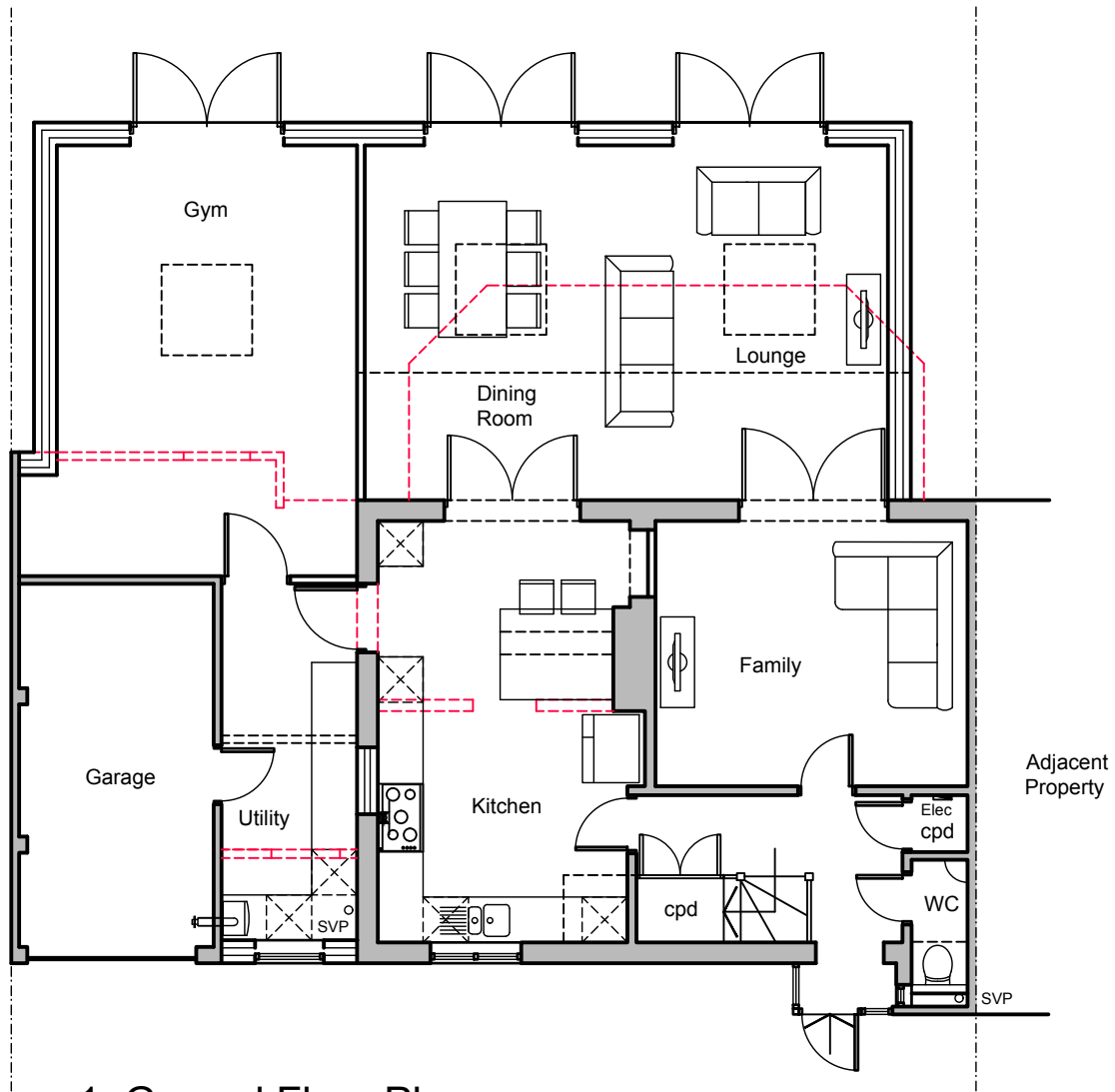
1. Ground Floor Plan
