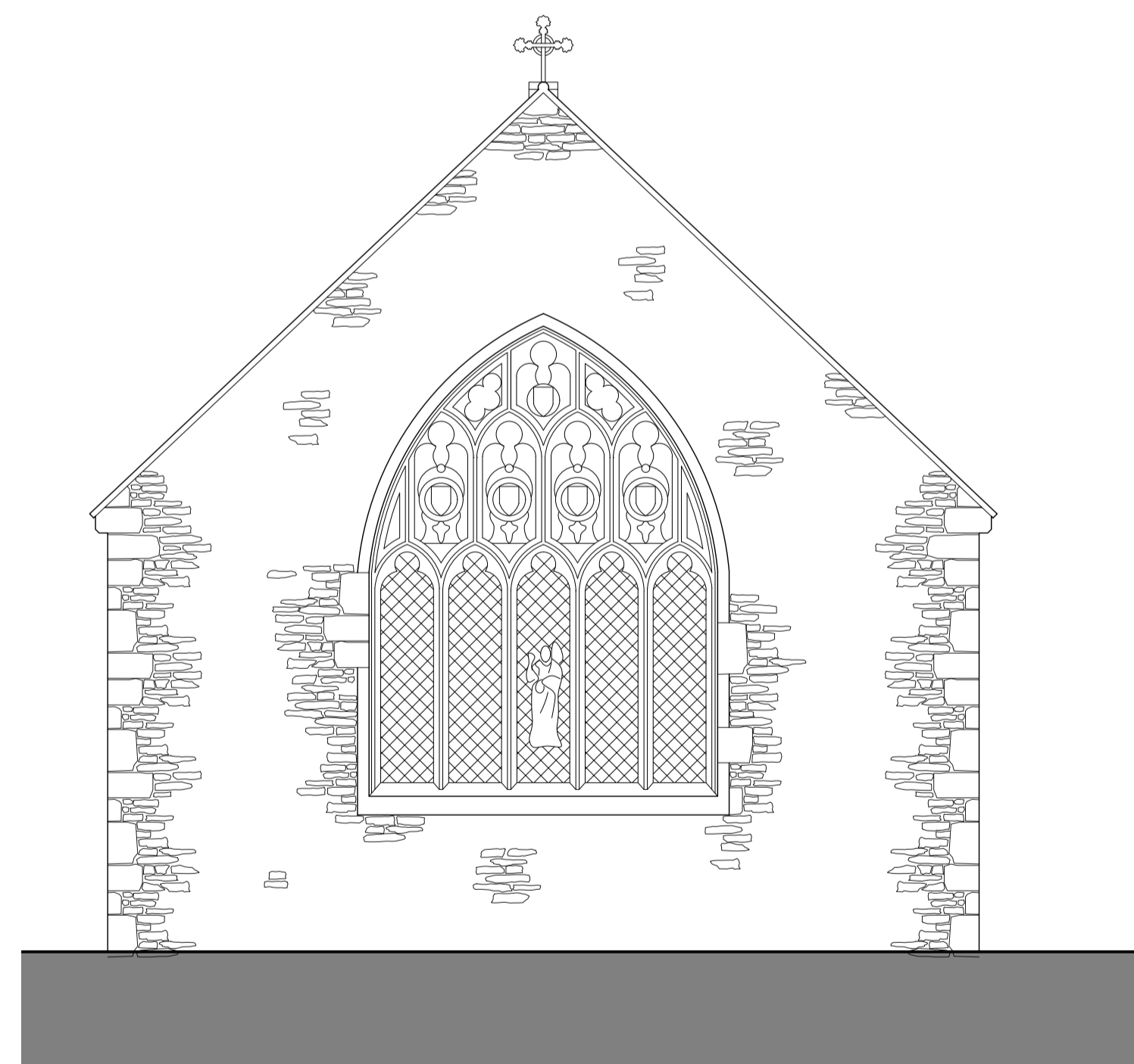
East Elevation
