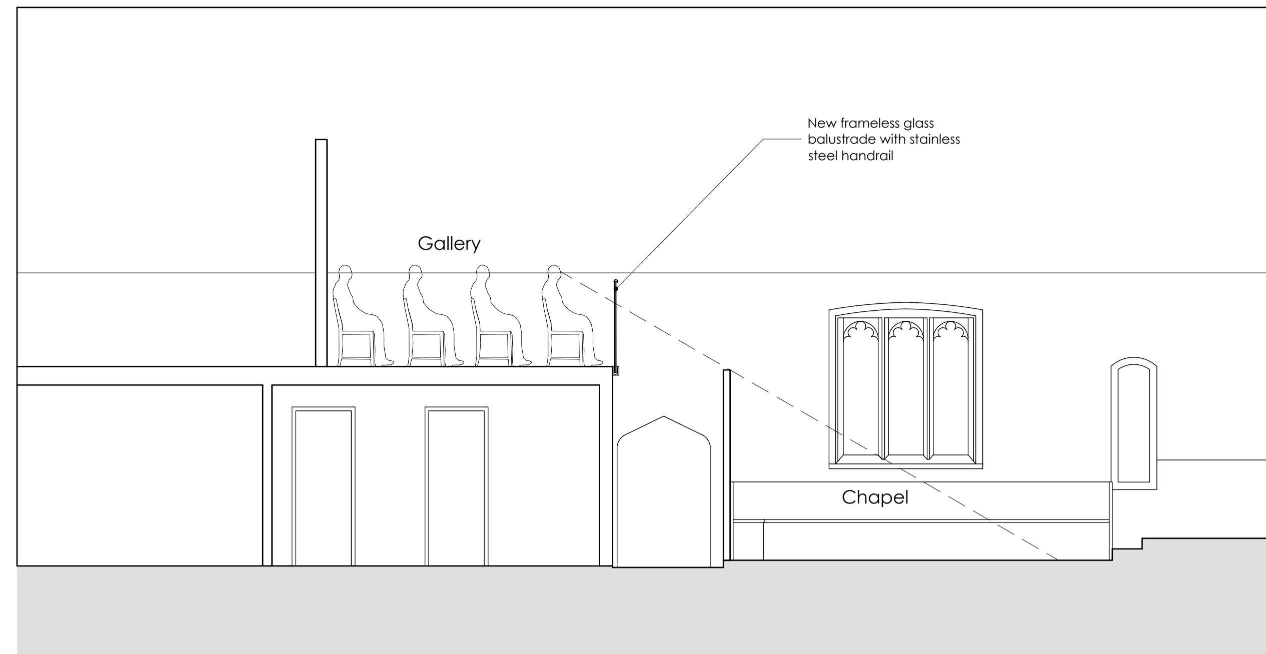
Section as Proposed
