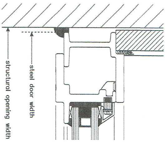
DOOR JAMB TO STRUCTURE
