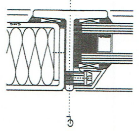
GLAZING BAR WITH KICK PANEL
