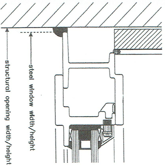
TOP HUNG TO STRUCTURE
