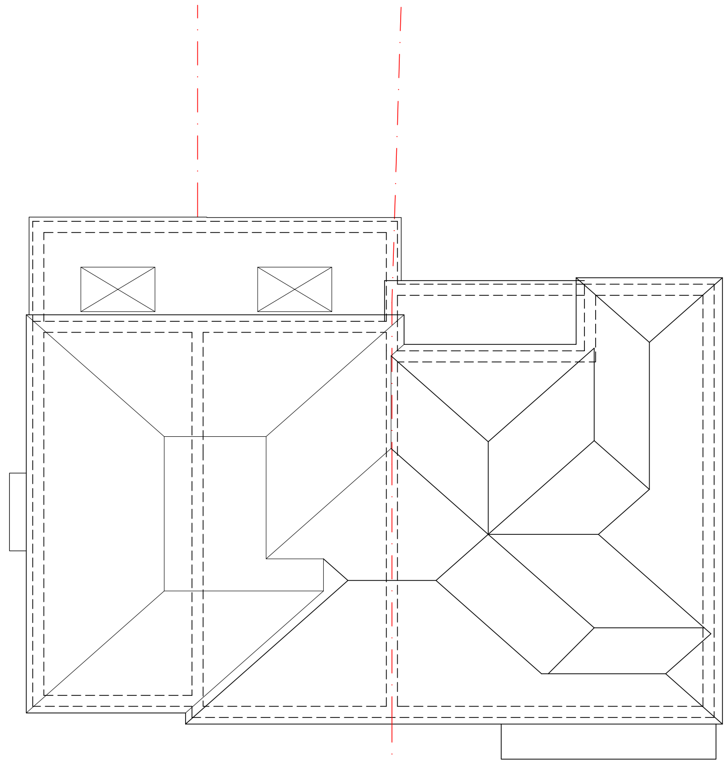
ROOF PLAN
