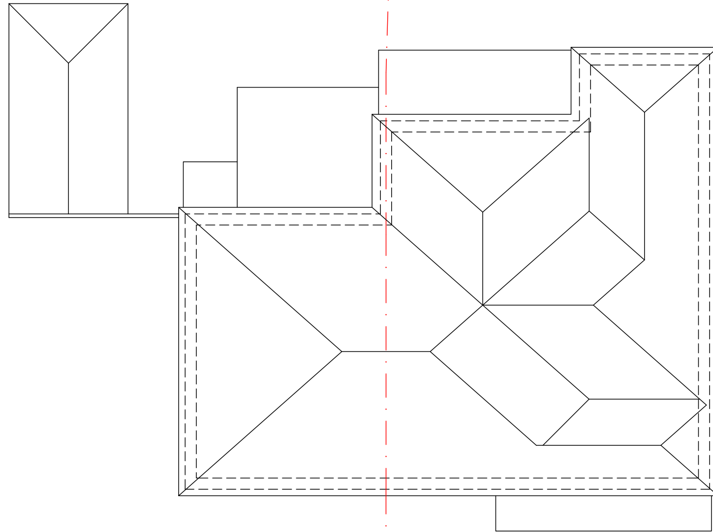
ROOF PLAN
