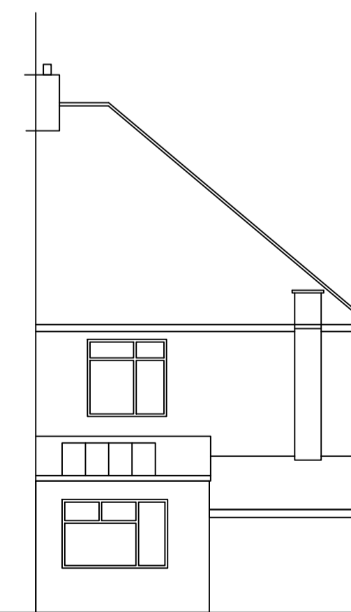
South Elevation @ 1:100
