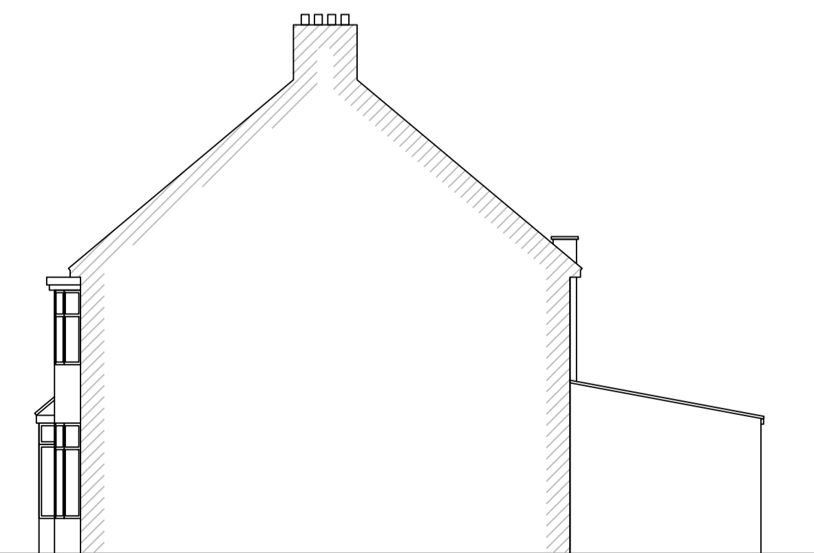
West Elevation @ 1:100
