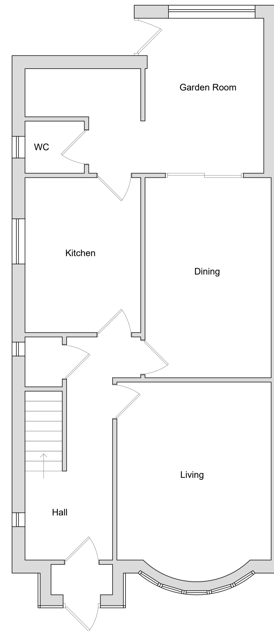
Ground Floor Plan @ 1:50
