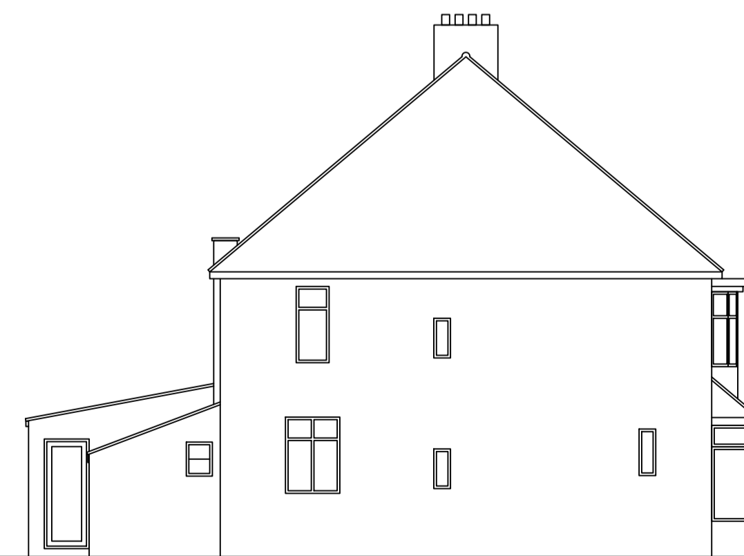
East Elevation @ 1:100
