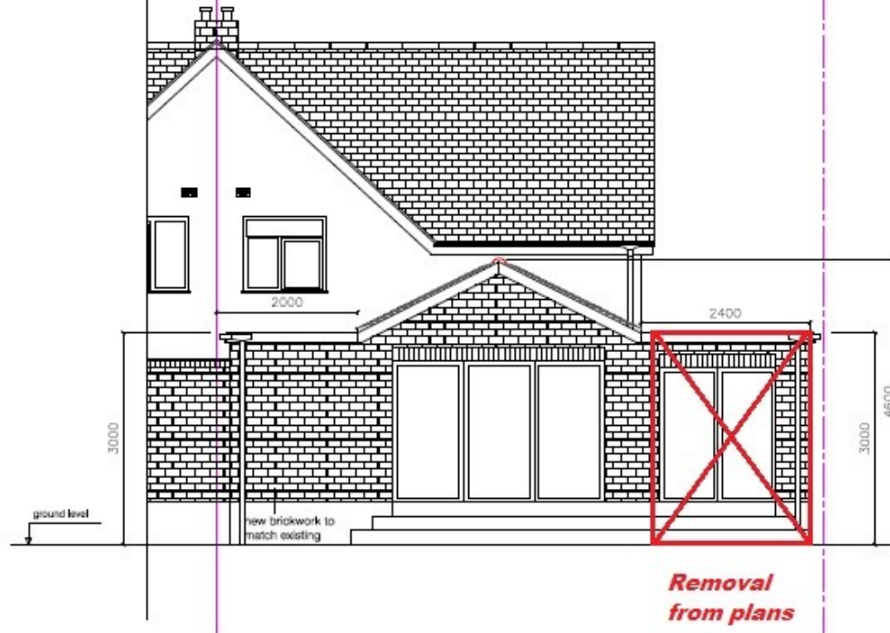
PROPOSED REAR ELEVATION PLAN
