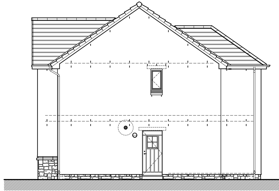
Gable Elevation
