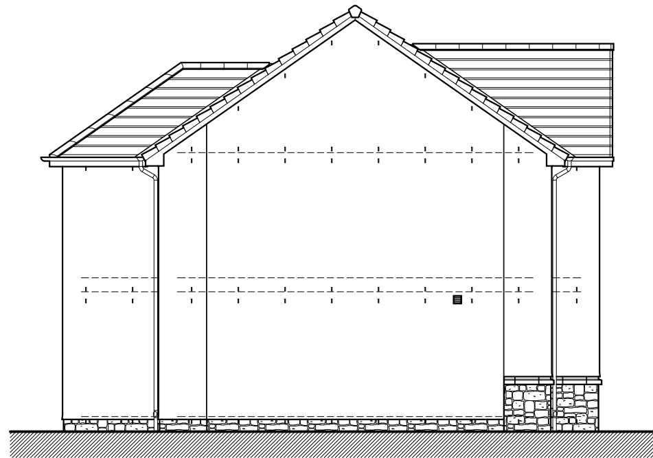
Gable Elevation
