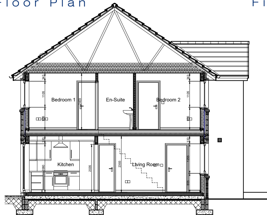
Typical Section
