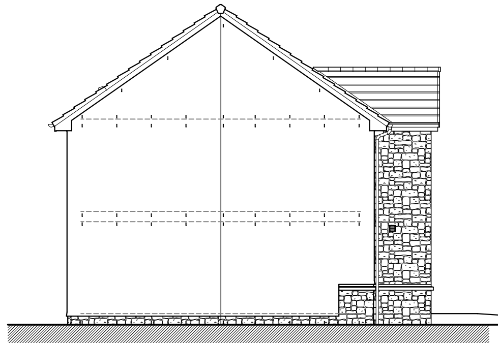
Gable Elevation
