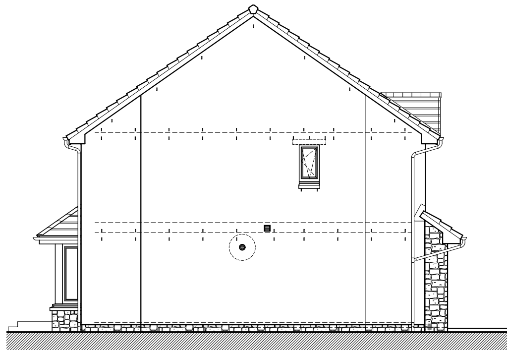
Gable Elevation
