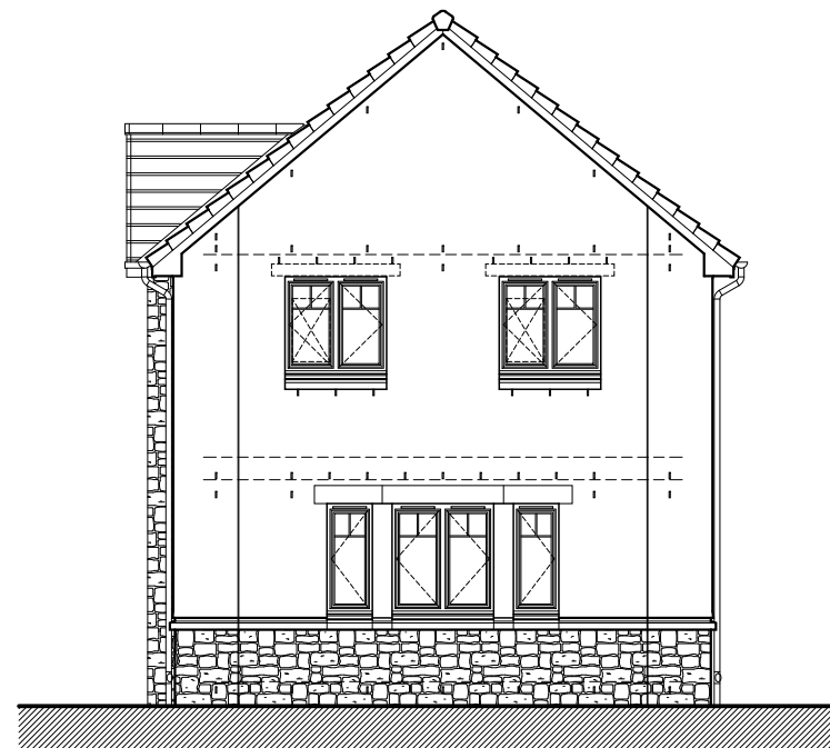
Gable Elevation
