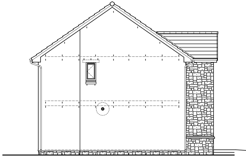
Gable Elevation
