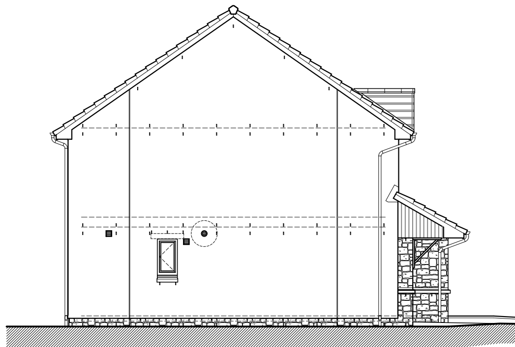
Gable Elevation
