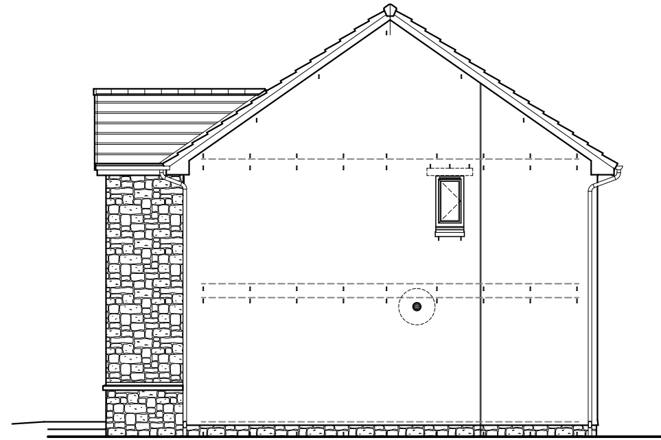
Gable Elevation
