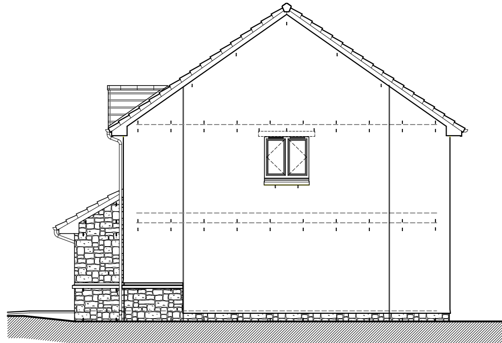
Gable Elevation
