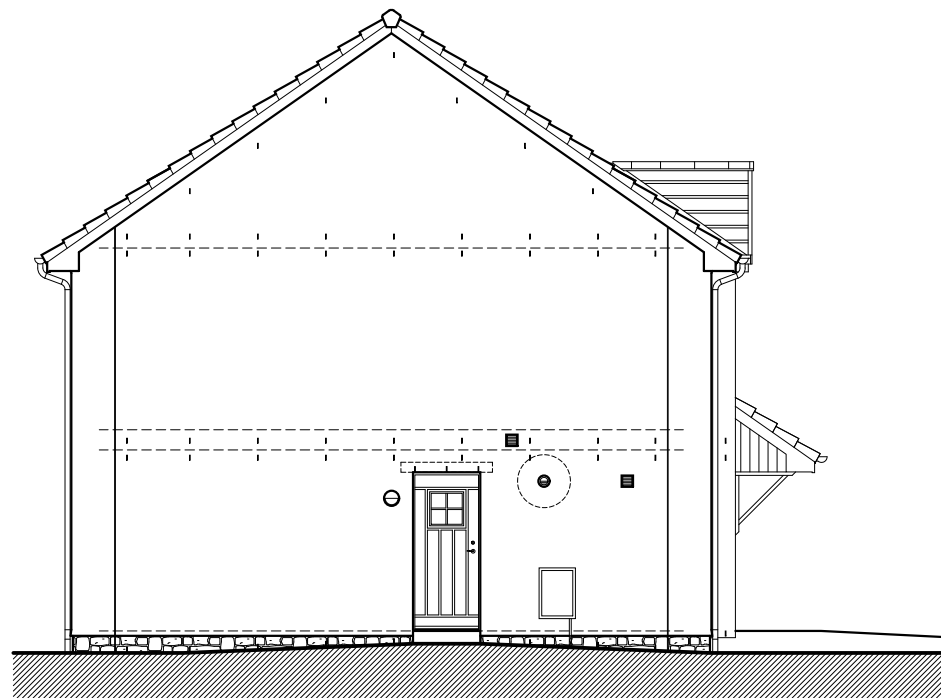
Gable Elevation
