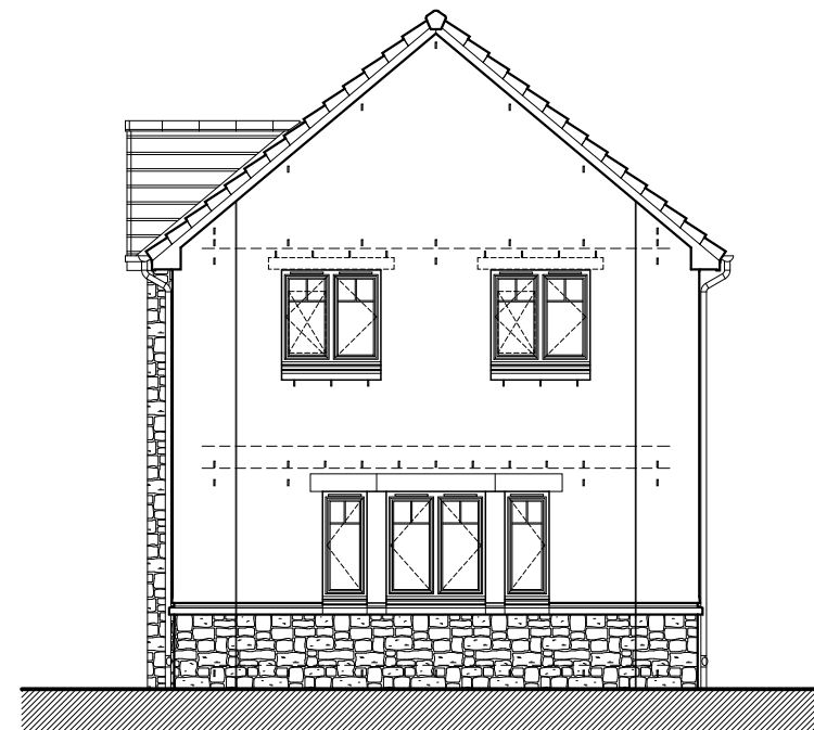
Gable Elevation
