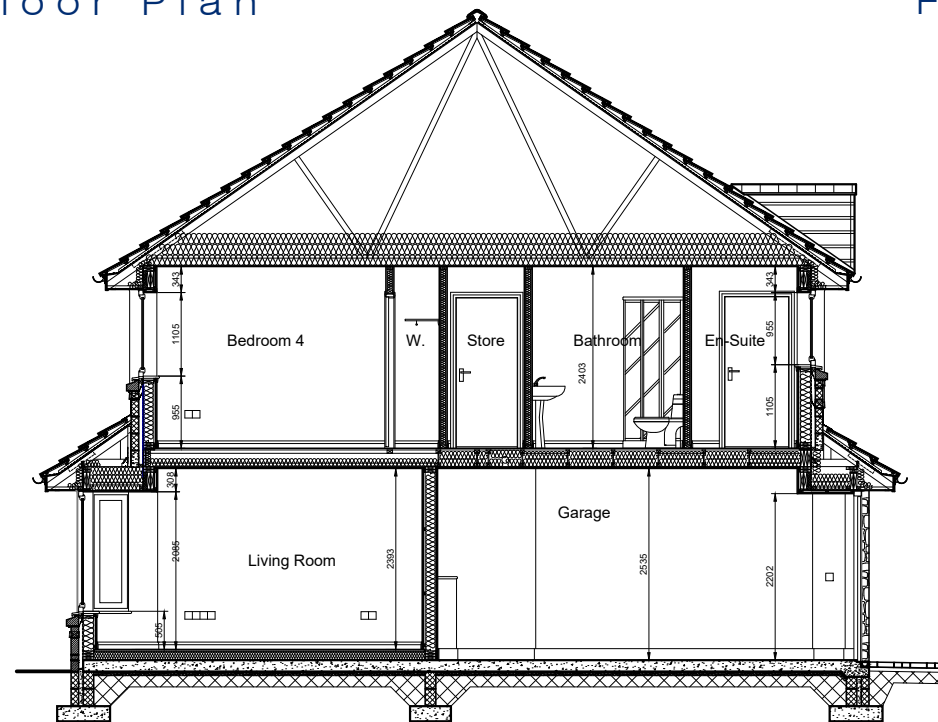
Typical Section
