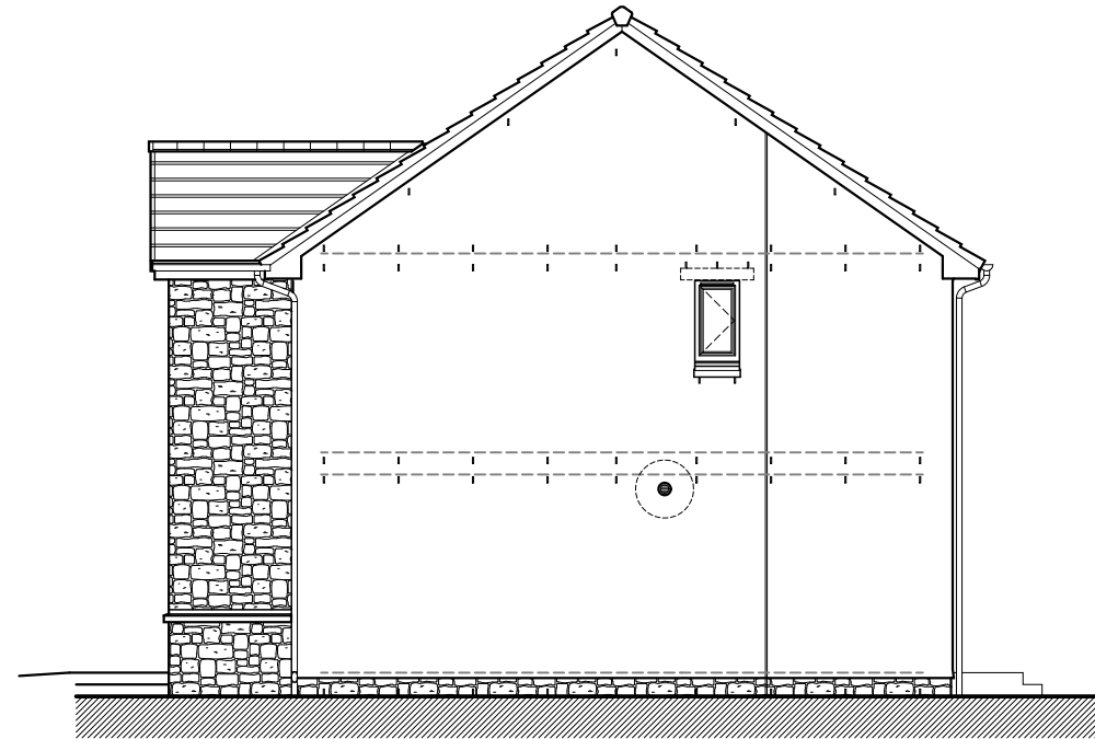
Gable Elevation
