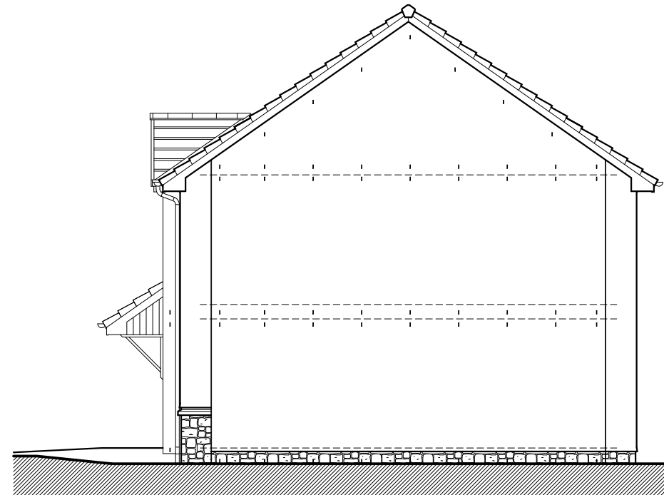
Gable Elevation
