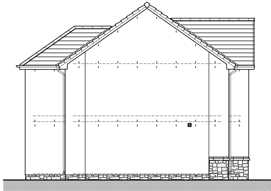
Gable Elevation
