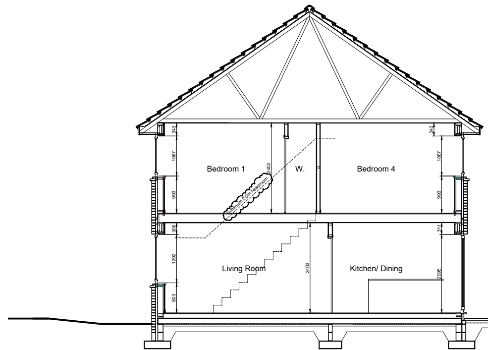
Typical Section
