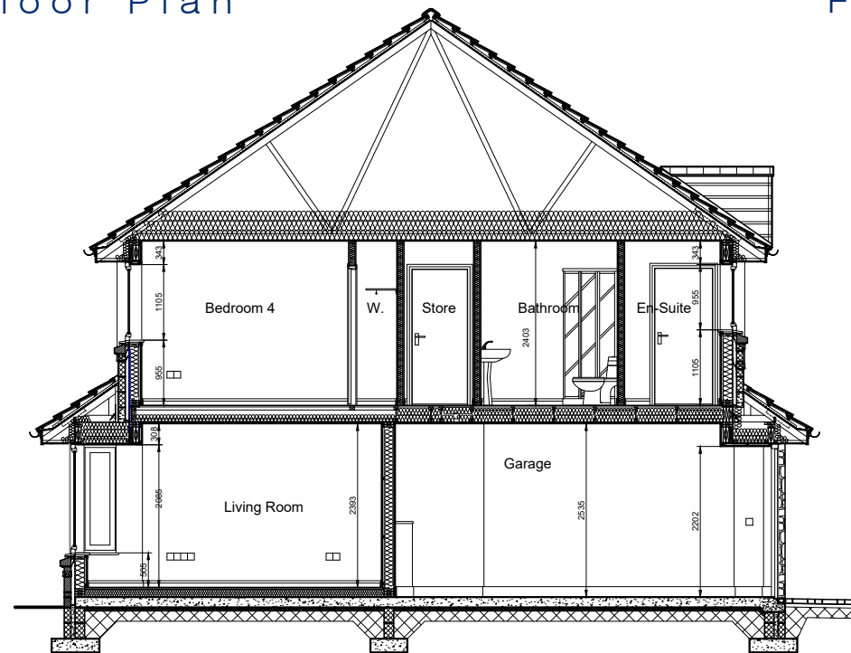
Typical Section
