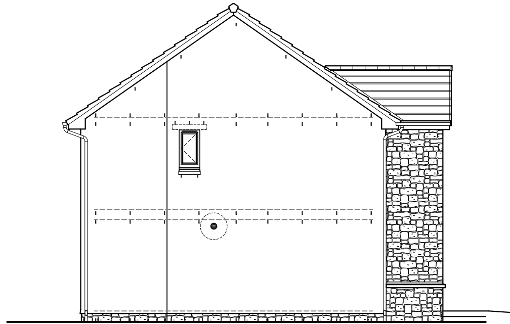
Gable Elevation
