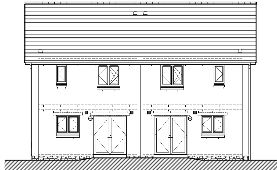
Rear Elevation
