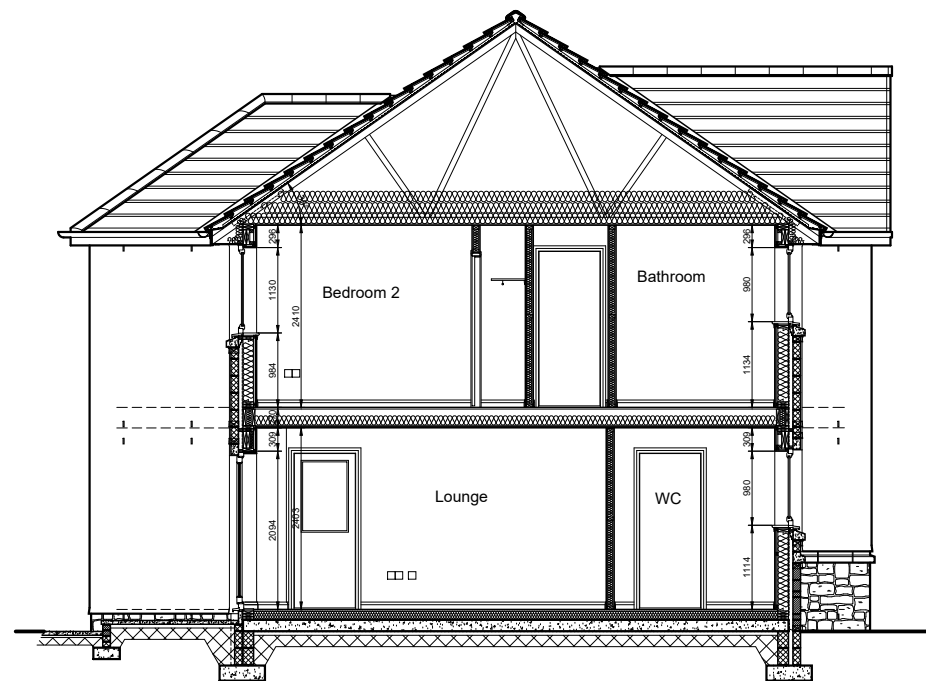
Typical Section
