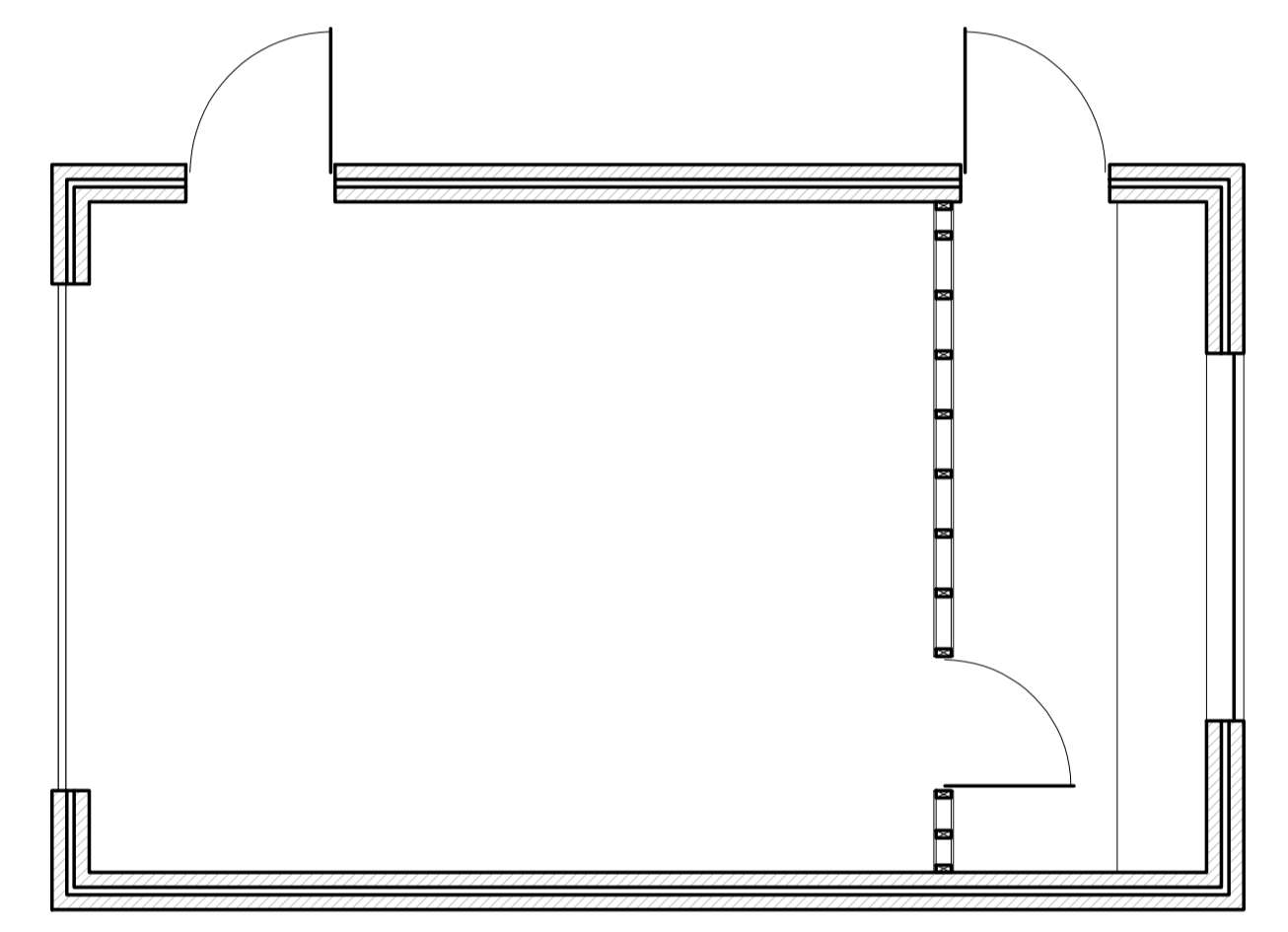
Proposed Garage Plan - 1/50
