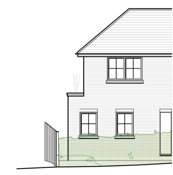
Proposed West Elevation Showing Boundary Fence following Site Levels - 1/100
