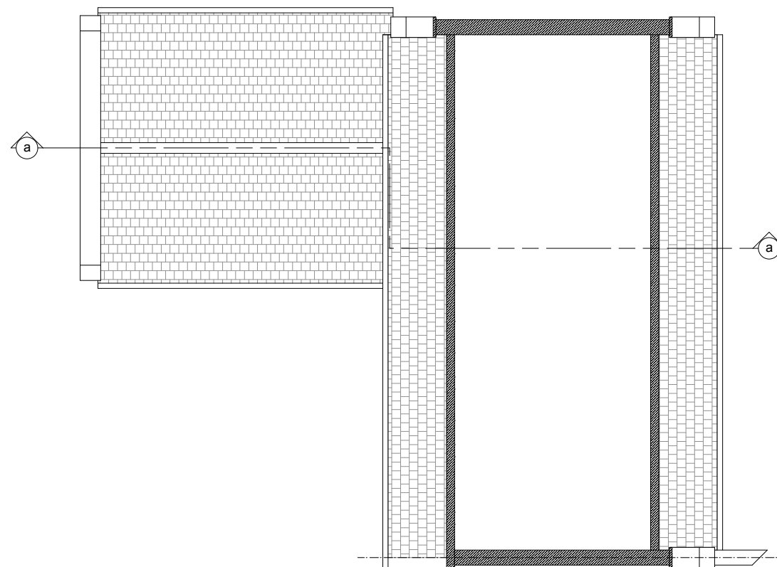
ATTIC PLAN
