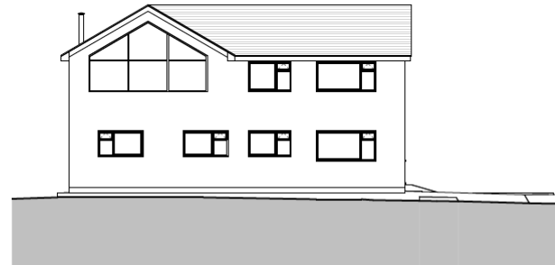
Front Elevation (West) 1:100
