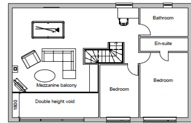
Level 1 - Proposed 1:100
