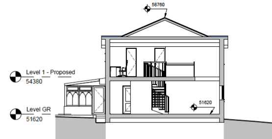
Section AA 1:100
