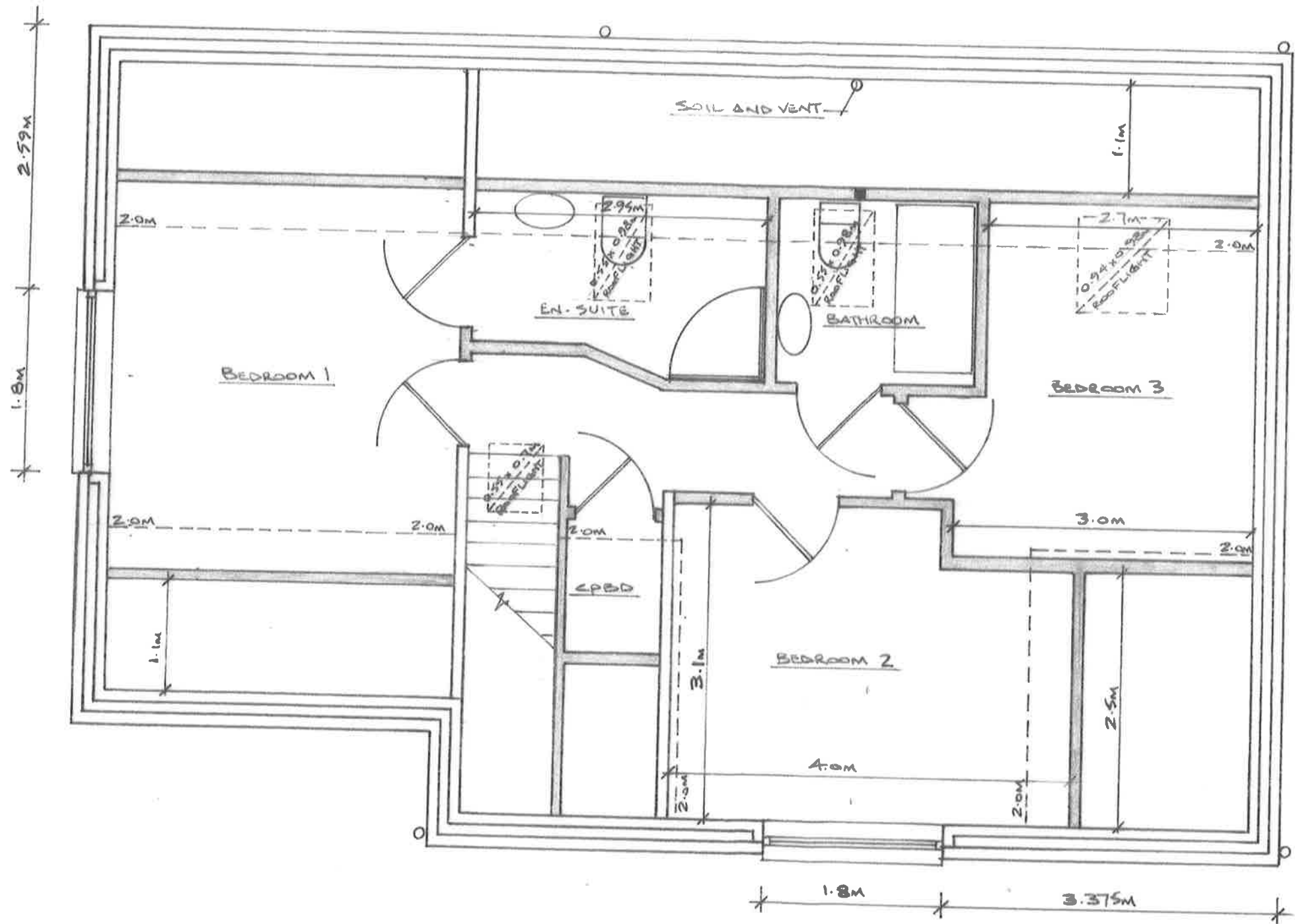
FIRST FLOOR LAYOUT 1:50
