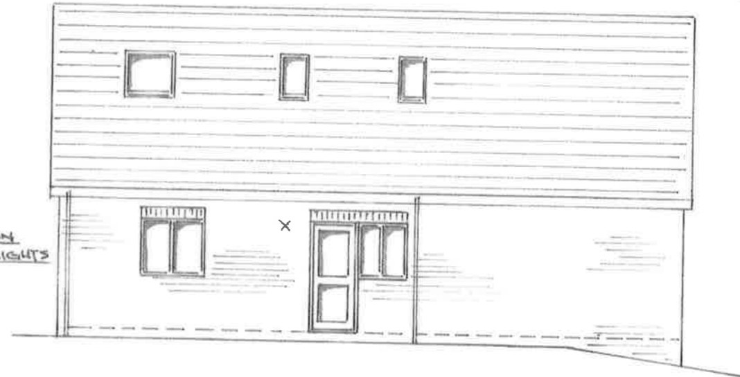
REAR ELEVATION (SE) 1:100
