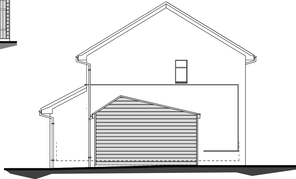
West elevation as proposed
