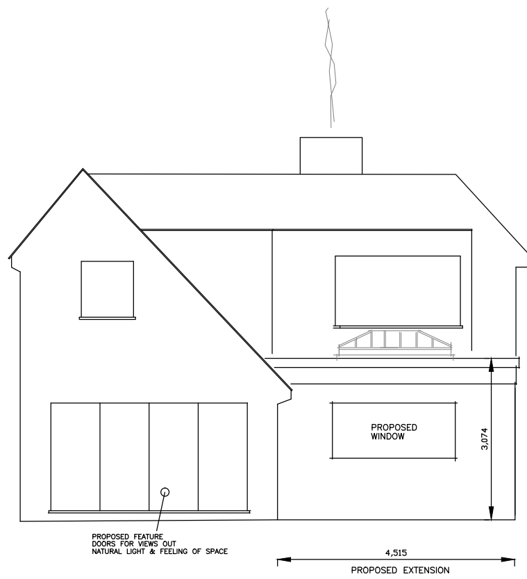
REAR ELEVATION
