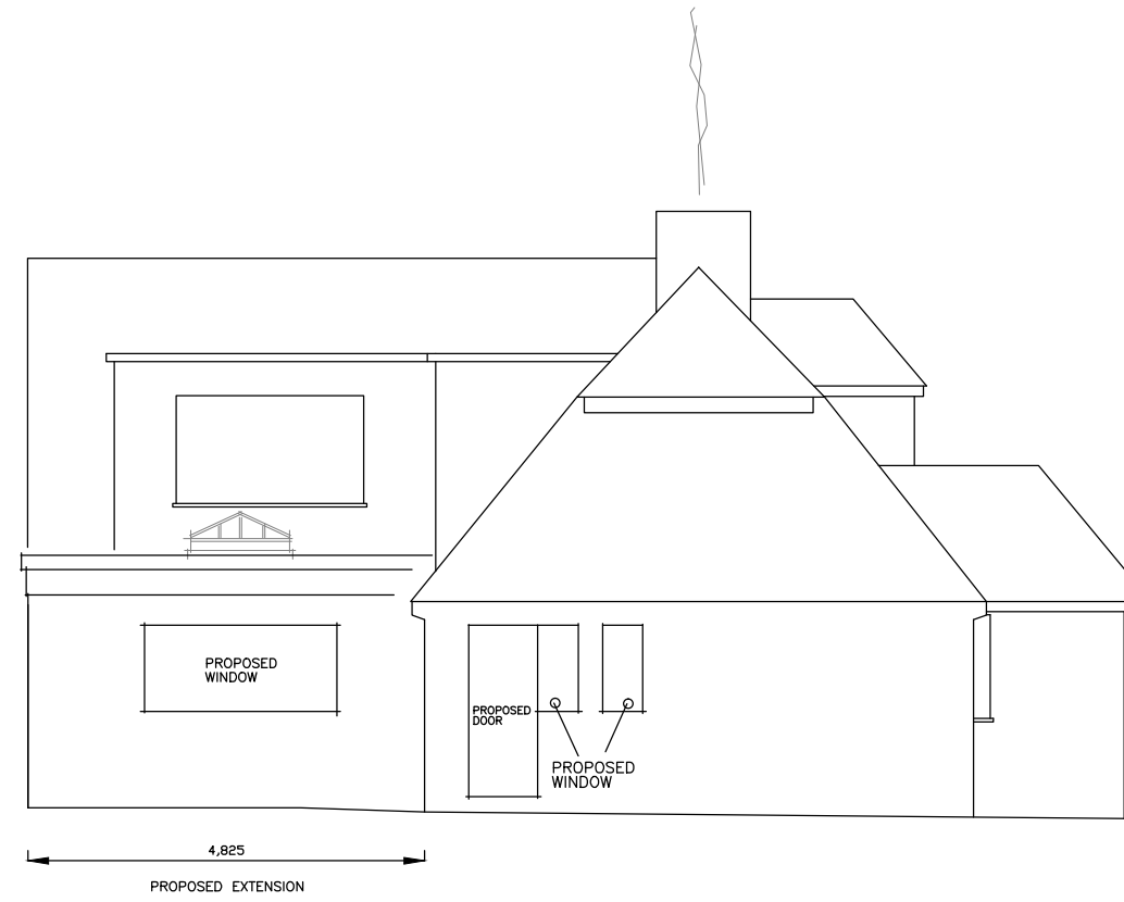
LEFT ELEVATION
