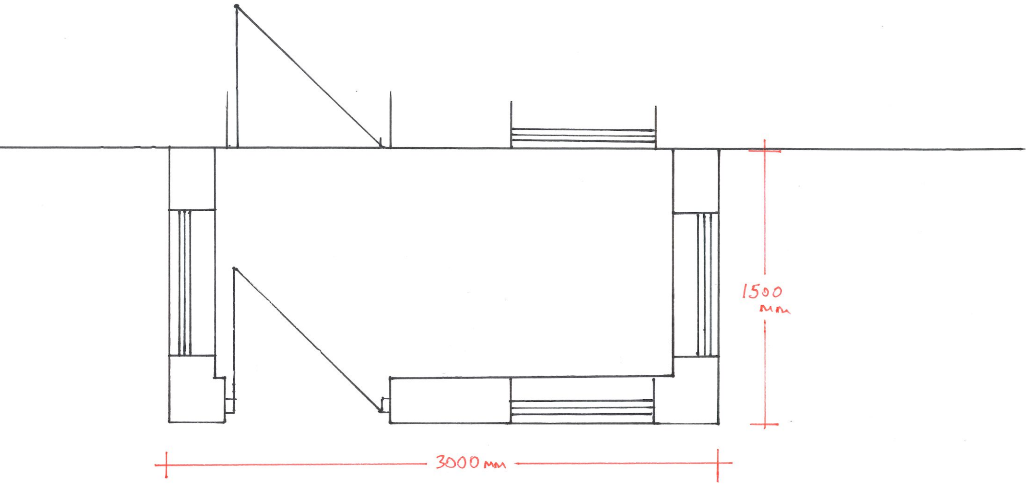
4. PLAN VIEW - PROPOSED 1:20
