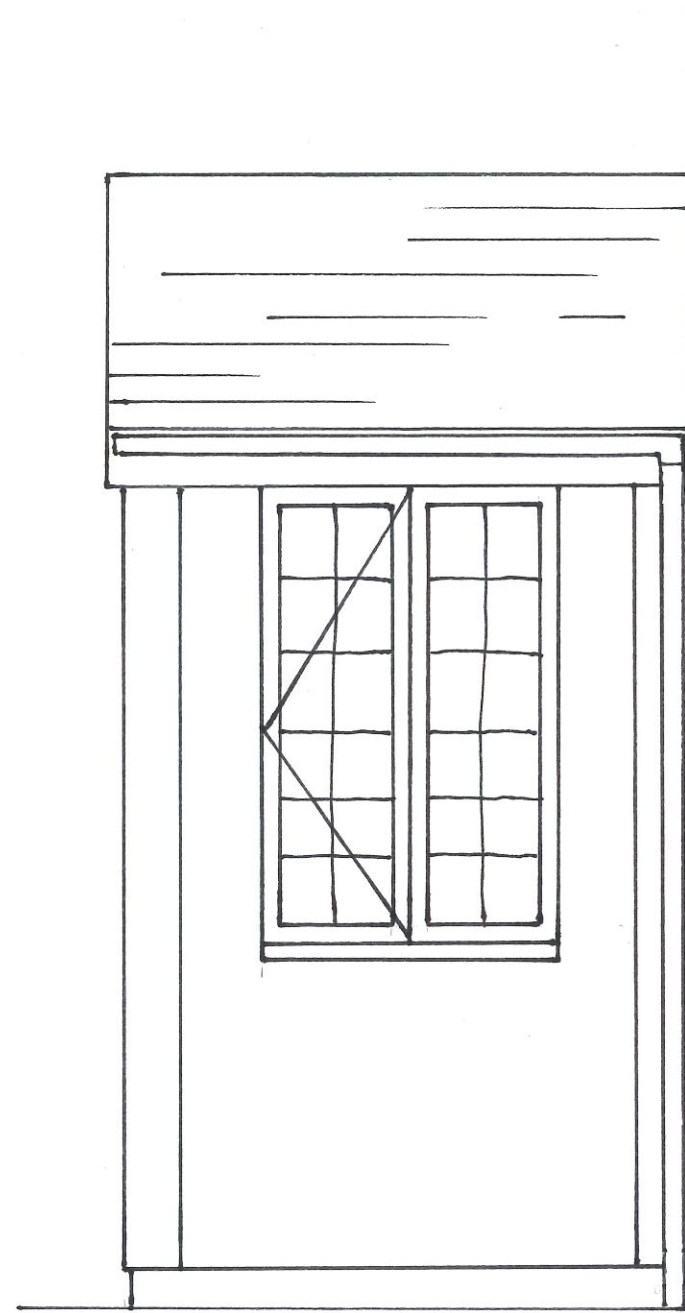
3. FRONT / REAR ELEVATION - PROPOSED 1:20
